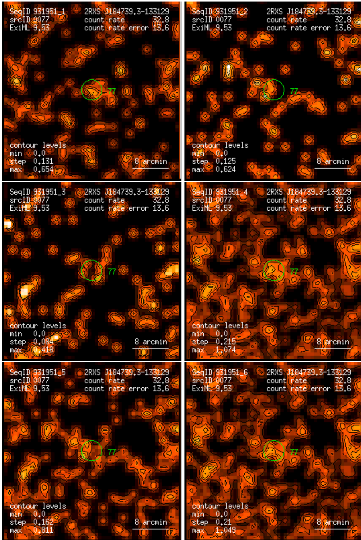
Figure 77: RASS 931951: detection 0077: band rate images, Gaussian filter: (1) PSPC channels 11 – 41, (2) 52 – 90, (3) 91 – 201, (4) 11 – 235, (5) 52 – 201, (6) 11 – 201. Broad band rates in counts/ks. Band rate contour levels in counts/ks/arcmin 2 .
