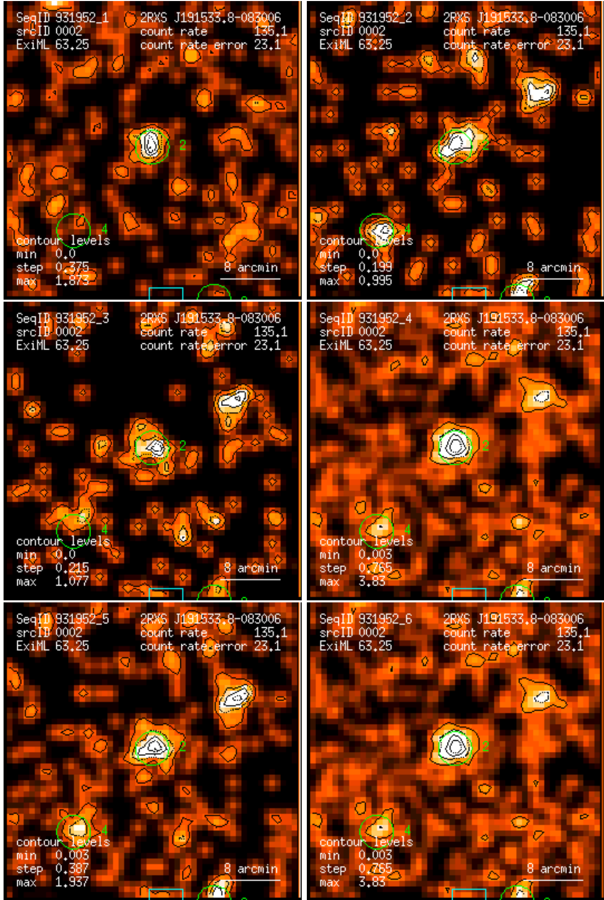
Figure 2: RASS 931952: detection 0002: band rate images, Gaussian filter: (1) PSPC channels 11 – 41, (2) 52 – 90, (3) 91 – 201, (4) 11 – 235, (5) 52 – 201, (6) 11 – 201. Broad band rates in counts/ks. Band rate contour levels in counts/ks/arcmin 2 .
