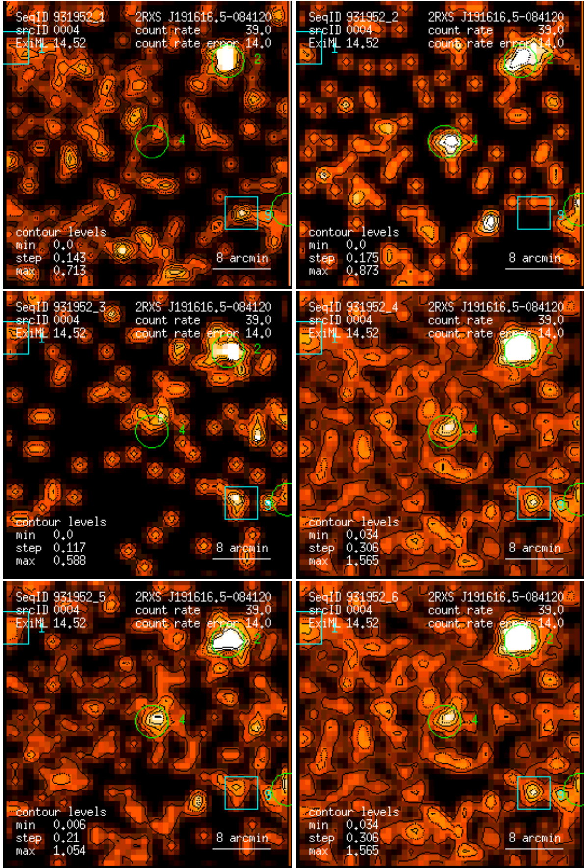
Figure 4: RASS 931952: detection 0004: band rate images, Gaussian filter: (1) PSPC channels 11 – 41, (2) 52 – 90, (3) 91 – 201, (4) 11 – 235, (5) 52 – 201, (6) 11 – 201. Broad band rates in counts/ks. Band rate contour levels in counts/ks/arcmin 2 .
