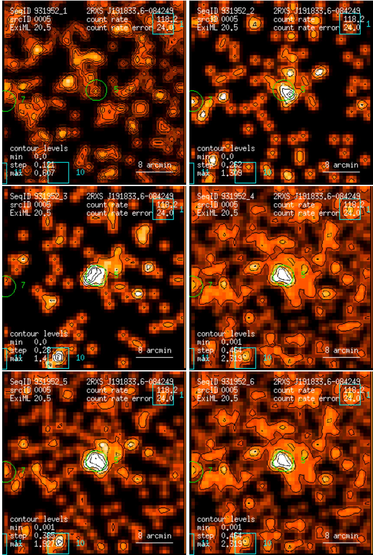
Figure 5: RASS 931952: detection 0005: band rate images, Gaussian filter: (1) PSPC channels 11 – 41, (2) 52 – 90, (3) 91 – 201, (4) 11 – 235, (5) 52 – 201, (6) 11 – 201. Broad band rates in counts/ks. Band rate contour levels in counts/ks/arcmin 2 .
