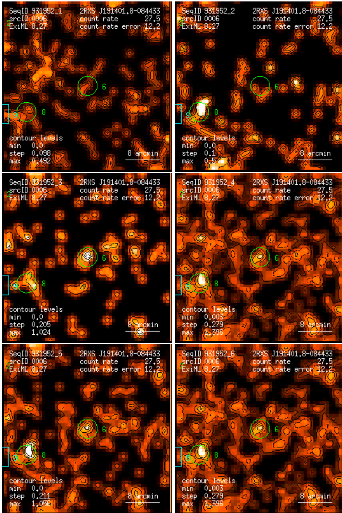
Figure 6: RASS 931952: detection 0006: band rate images, Gaussian filter: (1) PSPC channels 11 – 41, (2) 52 – 90, (3) 91 – 201, (4) 11 – 235, (5) 52 – 201, (6) 11 – 201. Broad band rates in counts/ks. Band rate contour levels in counts/ks/arcmin 2 .
