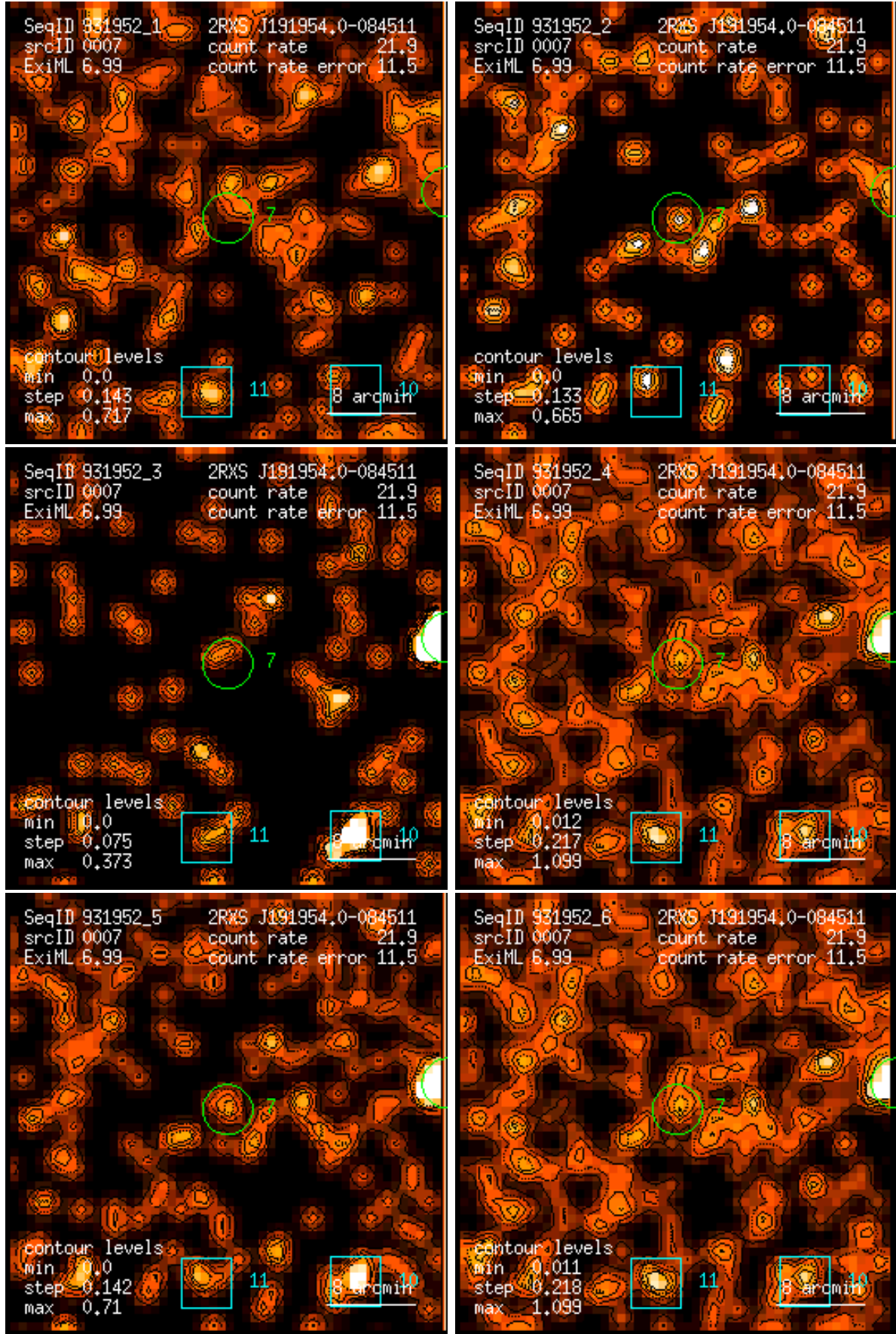
Figure 7: RASS 931952: detection 0007: band rate images, Gaussian filter: (1) PSPC channels 11 – 41, (2) 52 – 90, (3) 91 – 201, (4) 11 – 235, (5) 52 – 201, (6) 11 – 201. Broad band rates in counts/ks. Band rate contour levels in counts/ks/arcmin 2 .
