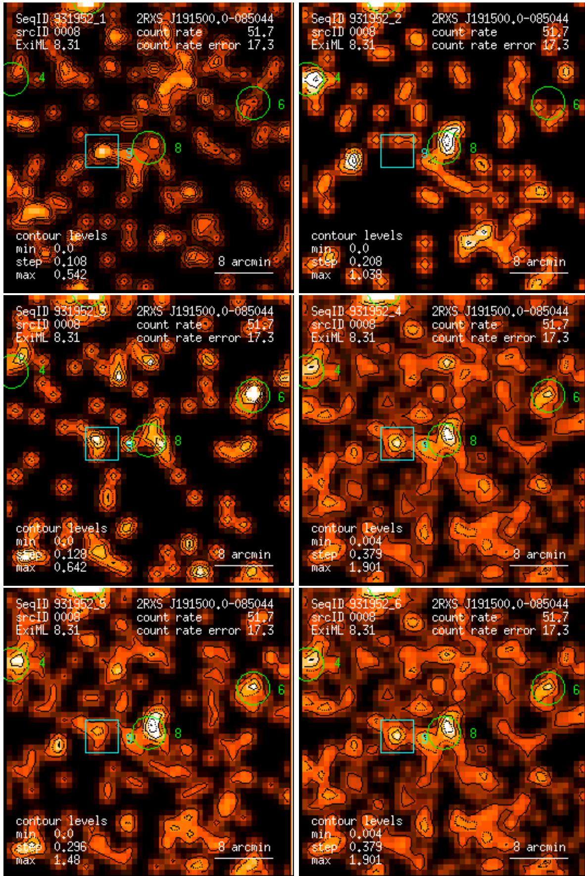
Figure 8: RASS 931952: detection 0008: band rate images, Gaussian filter: (1) PSPC channels 11 – 41, (2) 52 – 90, (3) 91 – 201, (4) 11 – 235, (5) 52 – 201, (6) 11 – 201. Broad band rates in counts/ks. Band rate contour levels in counts/ks/arcmin 2 .
