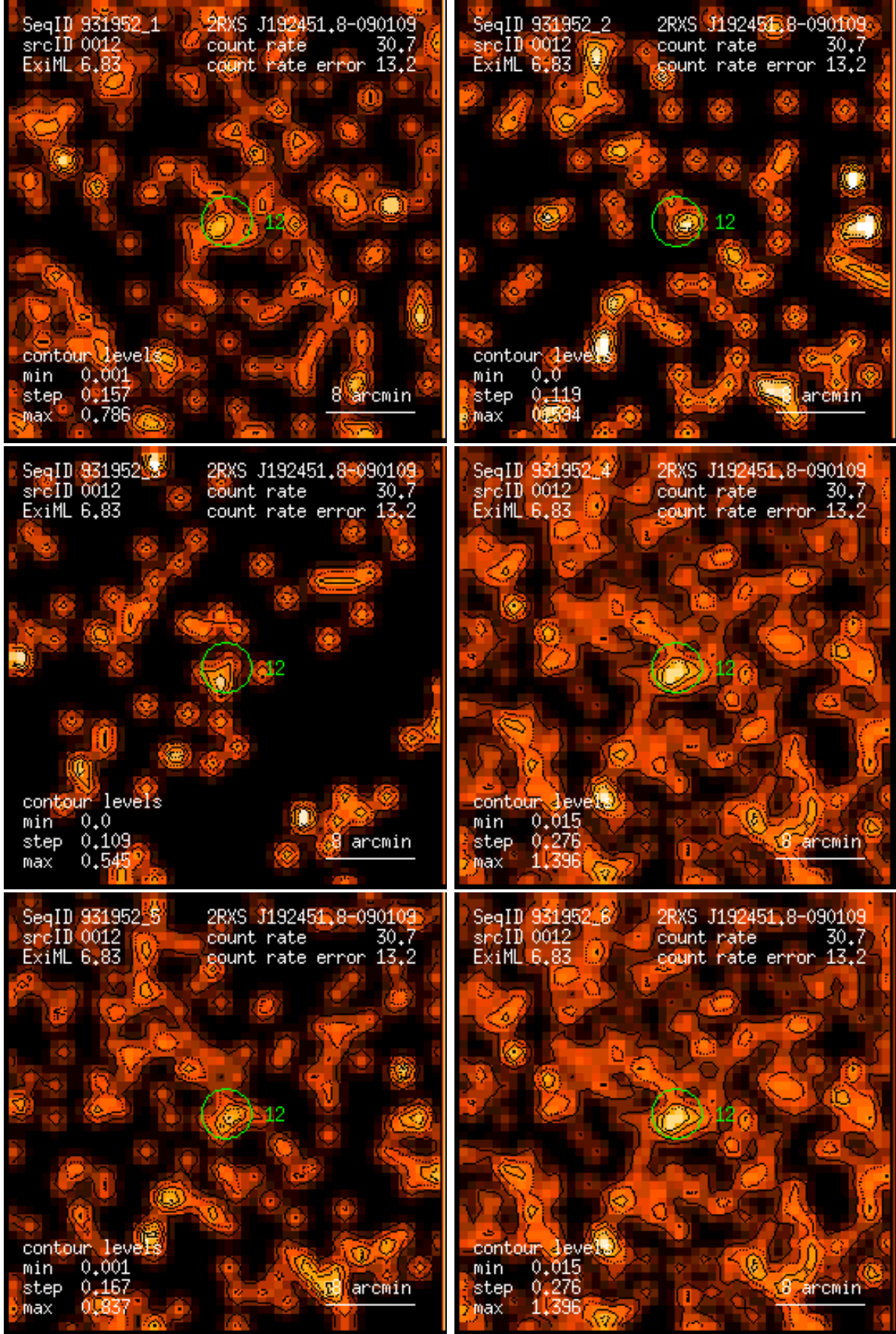
Figure 12: RASS 931952: detection 0012: band rate images, Gaussian filter: (1) PSPC channels 11 – 41, (2) 52 – 90, (3) 91 – 201, (4) 11 – 235, (5) 52 – 201, (6) 11 – 201. Broad band rates in counts/ks. Band rate contour levels in counts/ks/arcmin 2 .
