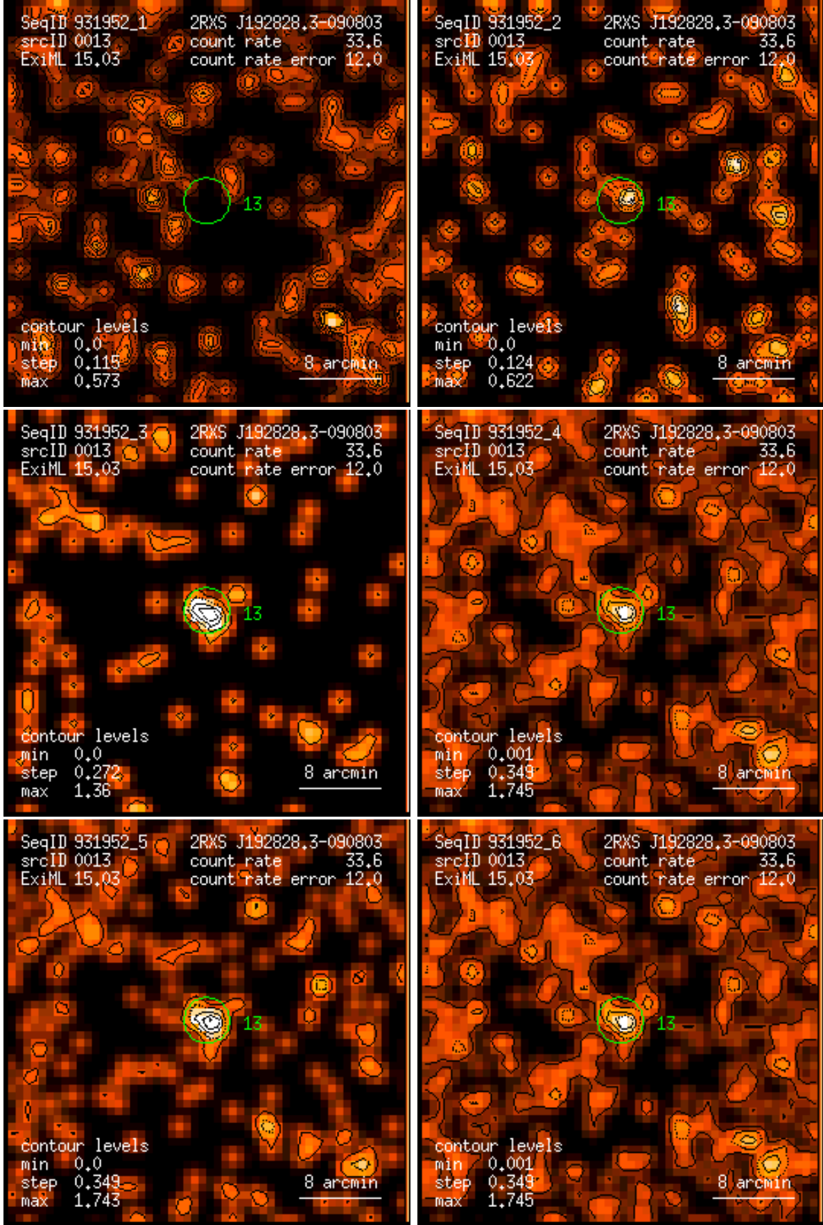
Figure 13: RASS 931952: detection 0013: band rate images, Gaussian filter: (1) PSPC channels 11 – 41, (2) 52 – 90, (3) 91 – 201, (4) 11 – 235, (5) 52 – 201, (6) 11 – 201. Broad band rates in counts/ks. Band rate contour levels in counts/ks/arcmin 2 .
