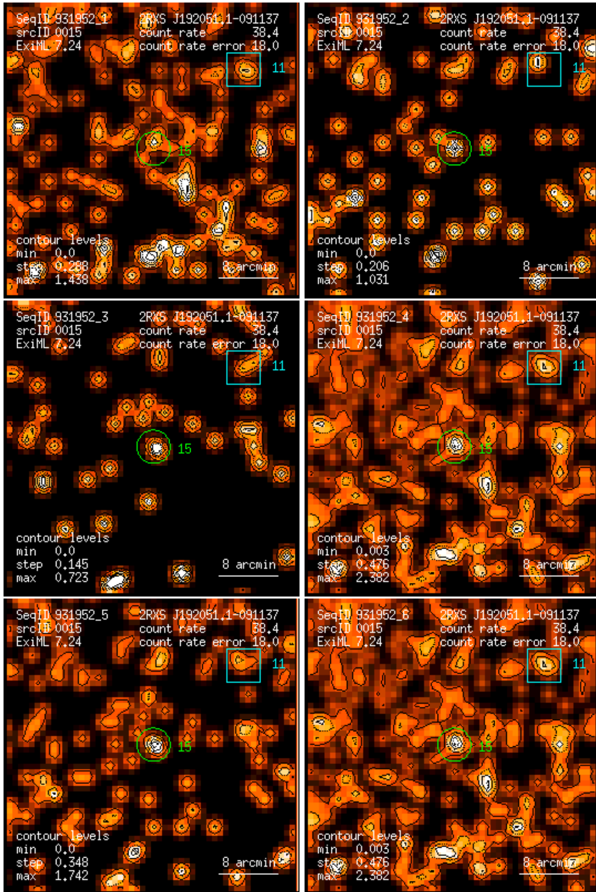
Figure 15: RASS 931952: detection 0015: band rate images, Gaussian filter: (1) PSPC channels 11 – 41, (2) 52 – 90, (3) 91 – 201, (4) 11 – 235, (5) 52 – 201, (6) 11 – 201. Broad band rates in counts/ks. Band rate contour levels in counts/ks/arcmin 2 .
