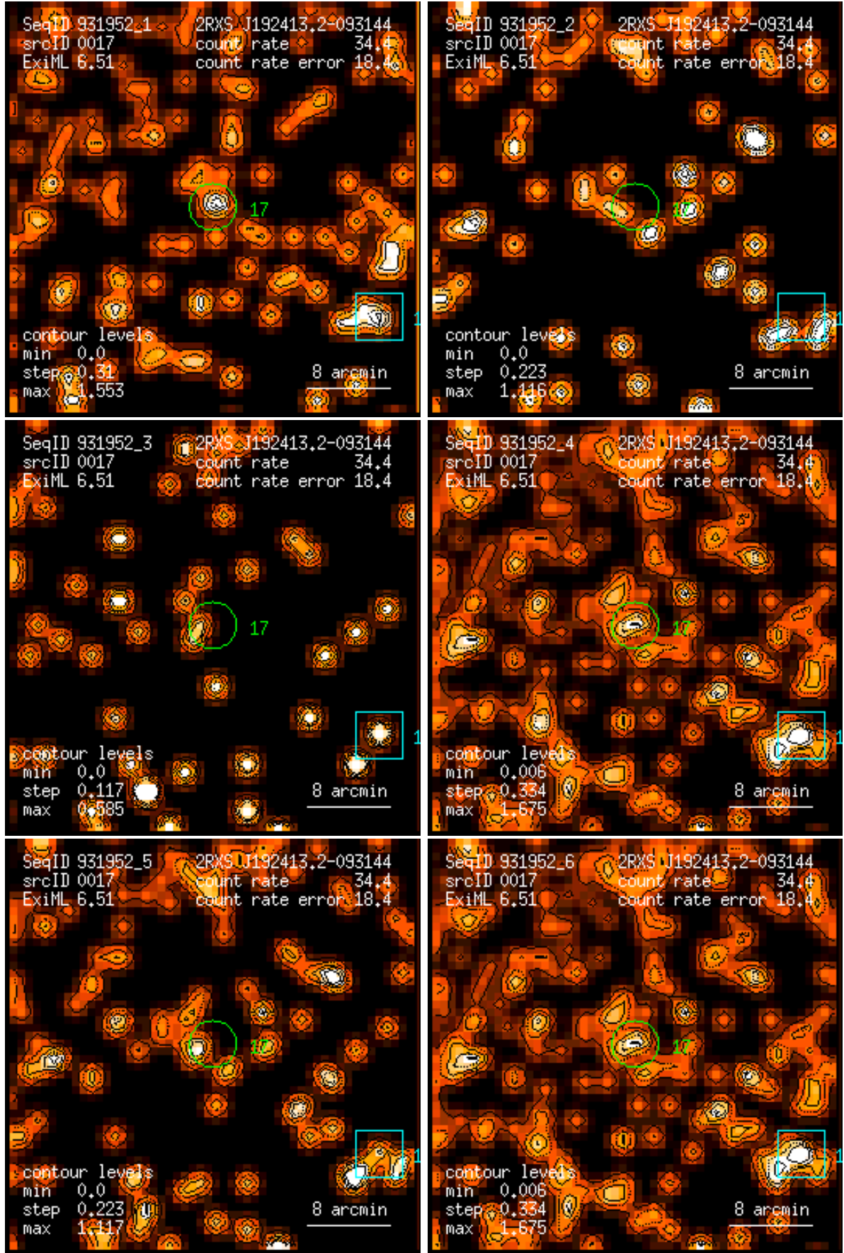
Figure 17: RASS 931952: detection 0017: band rate images, Gaussian filter: (1) PSPC channels 11 – 41, (2) 52 – 90, (3) 91 – 201, (4) 11 – 235, (5) 52 – 201, (6) 11 – 201. Broad band rates in counts/ks. Band rate contour levels in counts/ks/arcmin 2 .
