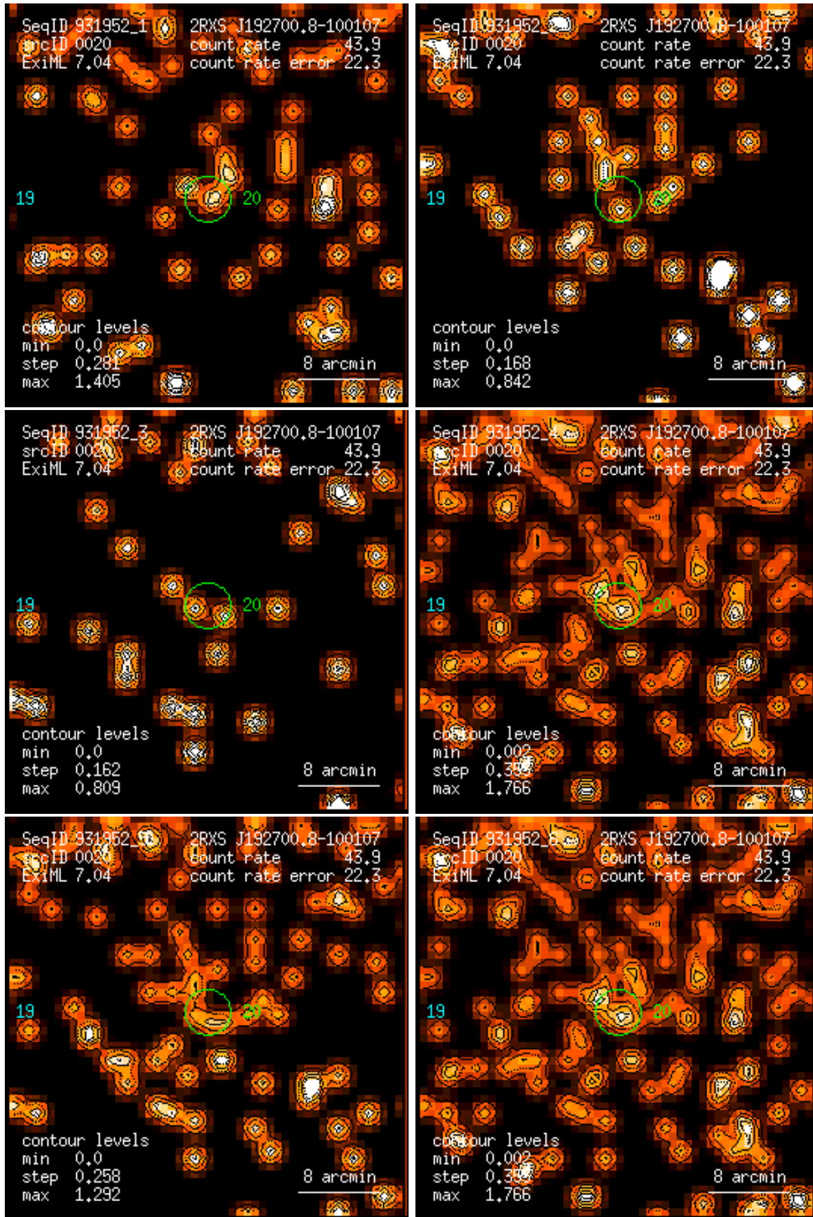
Figure 20: RASS 931952: detection 0020: band rate images, Gaussian filter: (1) PSPC channels 11 – 41, (2) 52 – 90, (3) 91 – 201, (4) 11 – 235, (5) 52 – 201, (6) 11 – 201. Broad band rates in counts/ks. Band rate contour levels in counts/ks/arcmin 2 .
