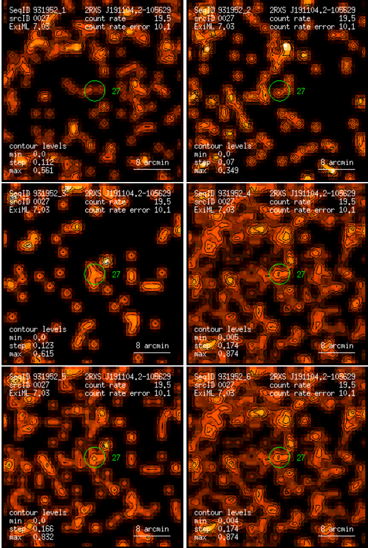
Figure 27: RASS 931952: detection 0027: band rate images, Gaussian filter: (1) PSPC channels 11 – 41, (2) 52 – 90, (3) 91 – 201, (4) 11 – 235, (5) 52 – 201, (6) 11 – 201. Broad band rates in counts/ks. Band rate contour levels in counts/ks/arcmin 2 .
