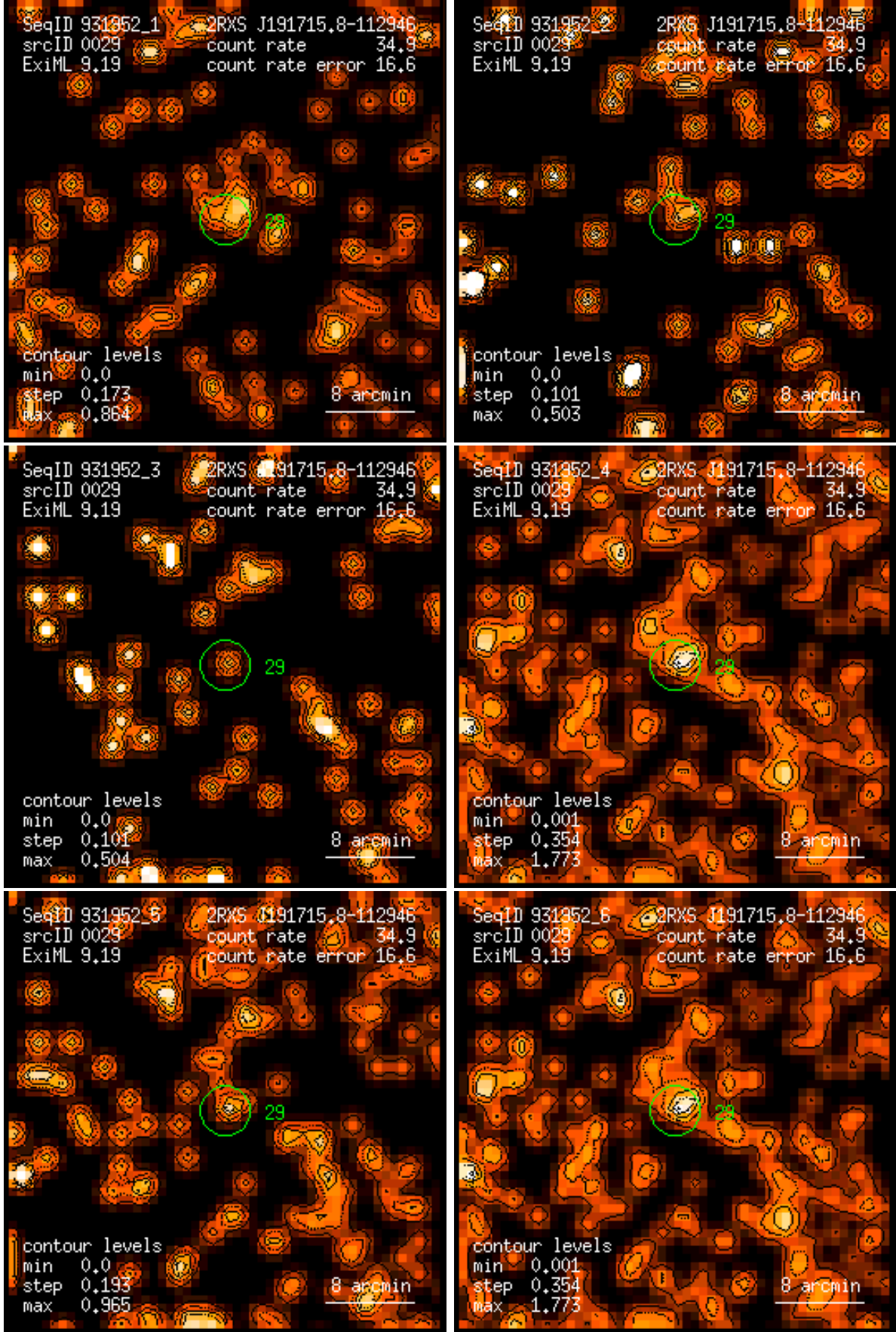
Figure 29: RASS 931952: detection 0029: band rate images, Gaussian filter: (1) PSPC channels 11 – 41, (2) 52 – 90, (3) 91 – 201, (4) 11 – 235, (5) 52 – 201, (6) 11 – 201. Broad band rates in counts/ks. Band rate contour levels in counts/ks/arcmin 2 .
