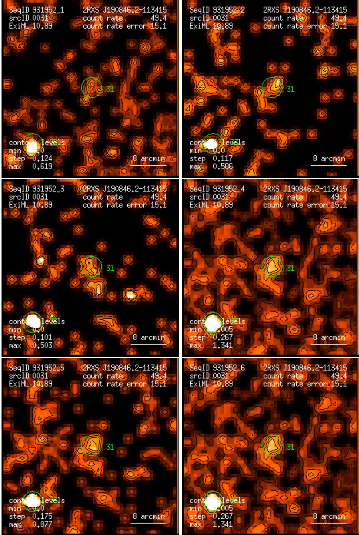
Figure 31: RASS 931952: detection 0031: band rate images, Gaussian filter: (1) PSPC channels 11 – 41, (2) 52 – 90, (3) 91 – 201, (4) 11 – 235, (5) 52 – 201, (6) 11 – 201. Broad band rates in counts/ks. Band rate contour levels in counts/ks/arcmin 2 .
