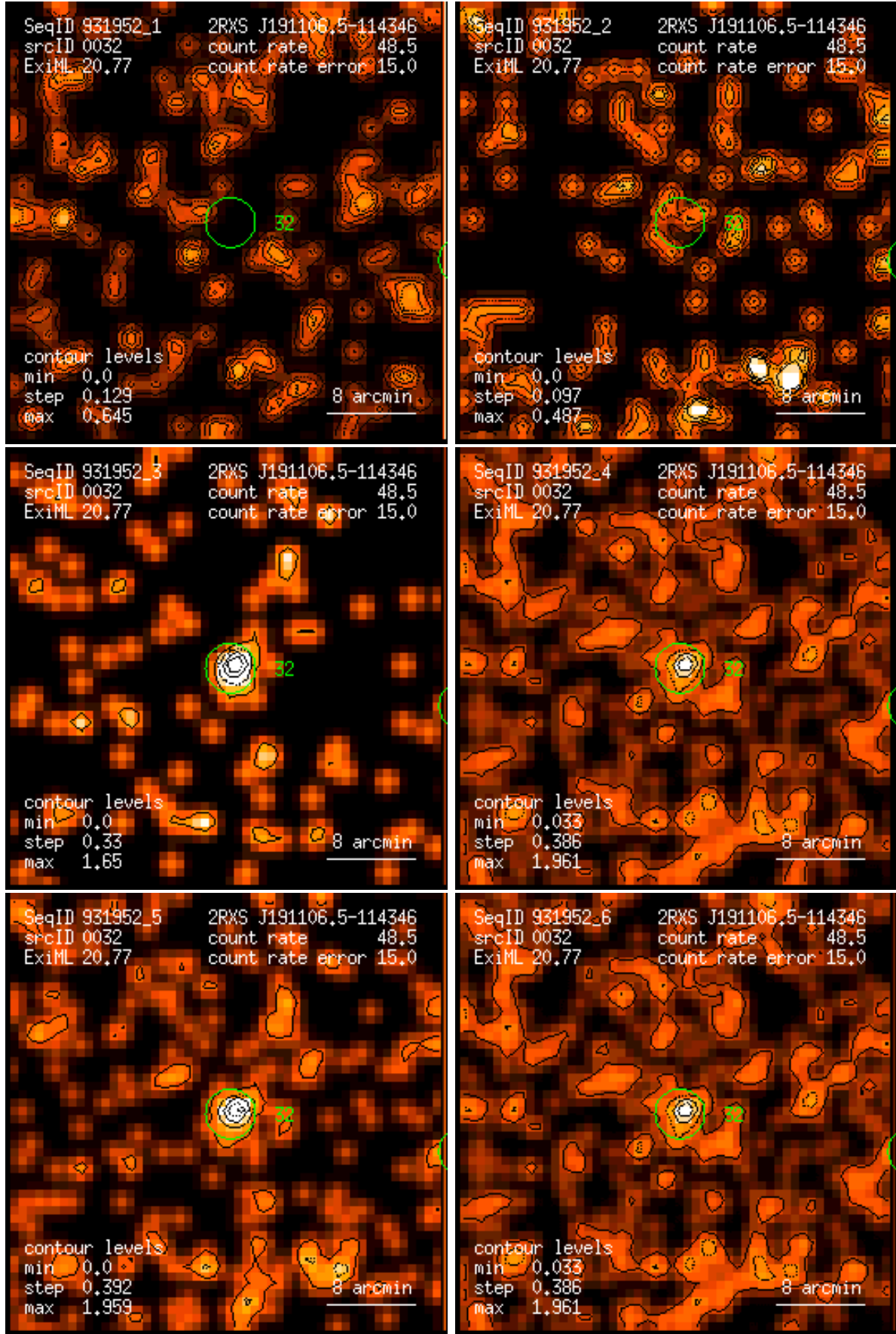
Figure 32: RASS 931952: detection 0032: band rate images, Gaussian filter: (1) PSPC channels 11 – 41, (2) 52 – 90, (3) 91 – 201, (4) 11 – 235, (5) 52 – 201, (6) 11 – 201. Broad band rates in counts/ks. Band rate contour levels in counts/ks/arcmin 2 .
