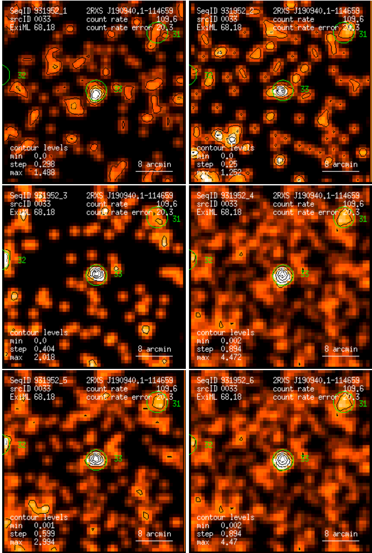
Figure 33: RASS 931952: detection 0033: band rate images, Gaussian filter: (1) PSPC channels 11 – 41, (2) 52 – 90, (3) 91 – 201, (4) 11 – 235, (5) 52 – 201, (6) 11 – 201. Broad band rates in counts/ks. Band rate contour levels in counts/ks/arcmin 2 .
