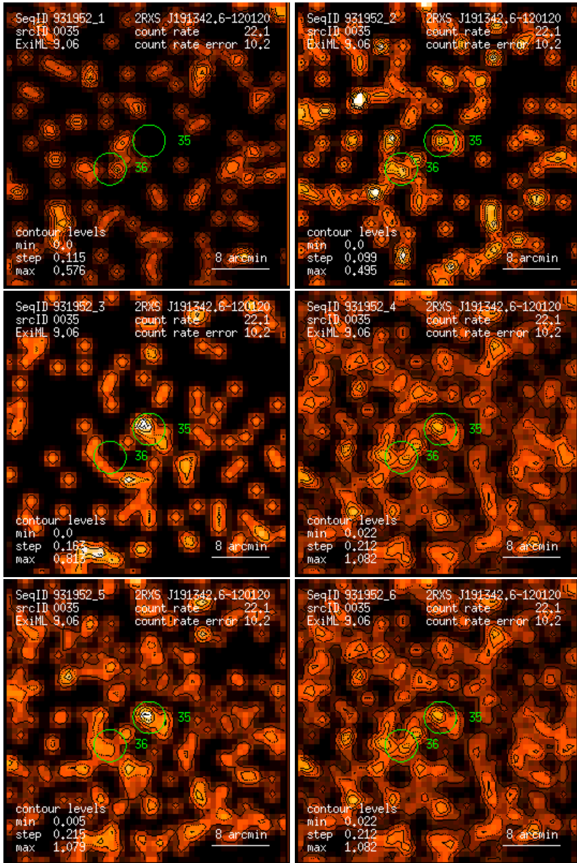
Figure 35: RASS 931952: detection 0035: band rate images, Gaussian filter: (1) PSPC channels 11 – 41, (2) 52 – 90, (3) 91 – 201, (4) 11 – 235, (5) 52 – 201, (6) 11 – 201. Broad band rates in counts/ks. Band rate contour levels in counts/ks/arcmin 2 .
