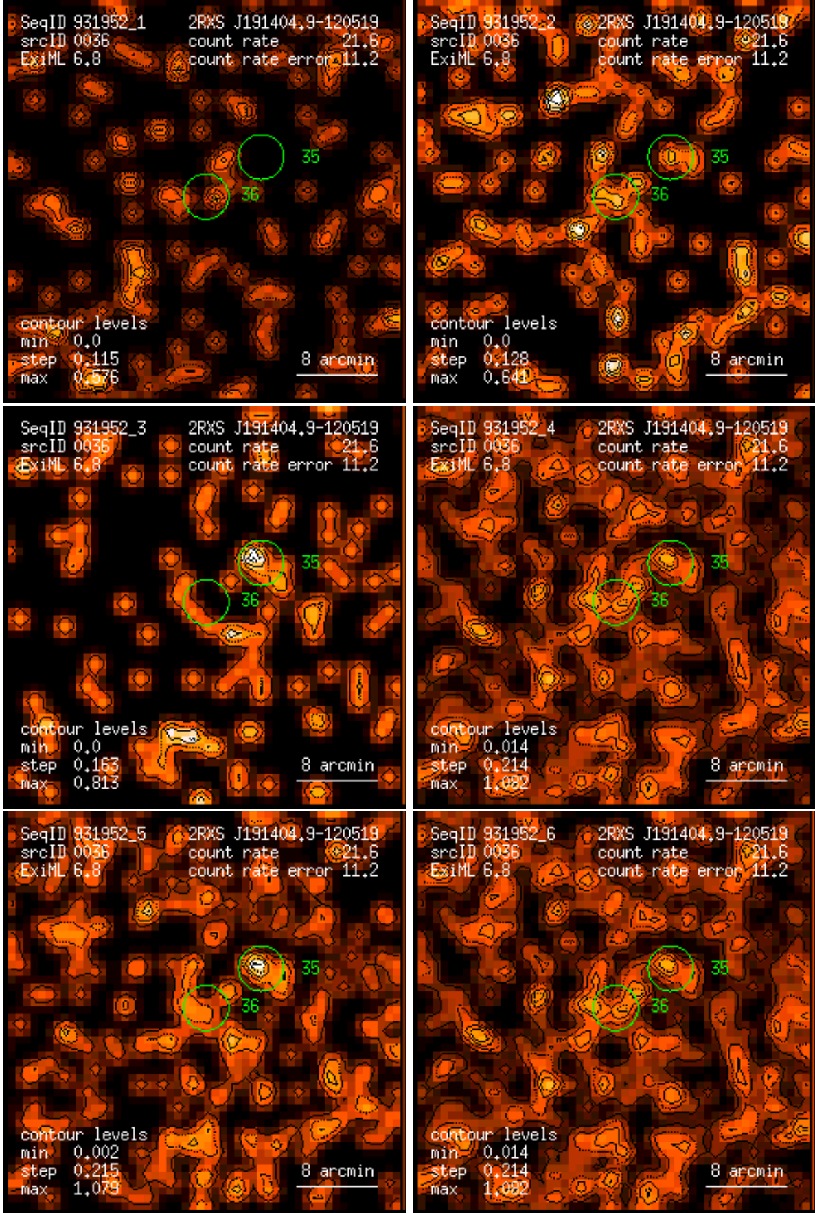
Figure 36: RASS 931952: detection 0036: band rate images, Gaussian filter: (1) PSPC channels 11 – 41, (2) 52 – 90, (3) 91 – 201, (4) 11 – 235, (5) 52 – 201, (6) 11 – 201. Broad band rates in counts/ks. Band rate contour levels in counts/ks/arcmin 2 .
