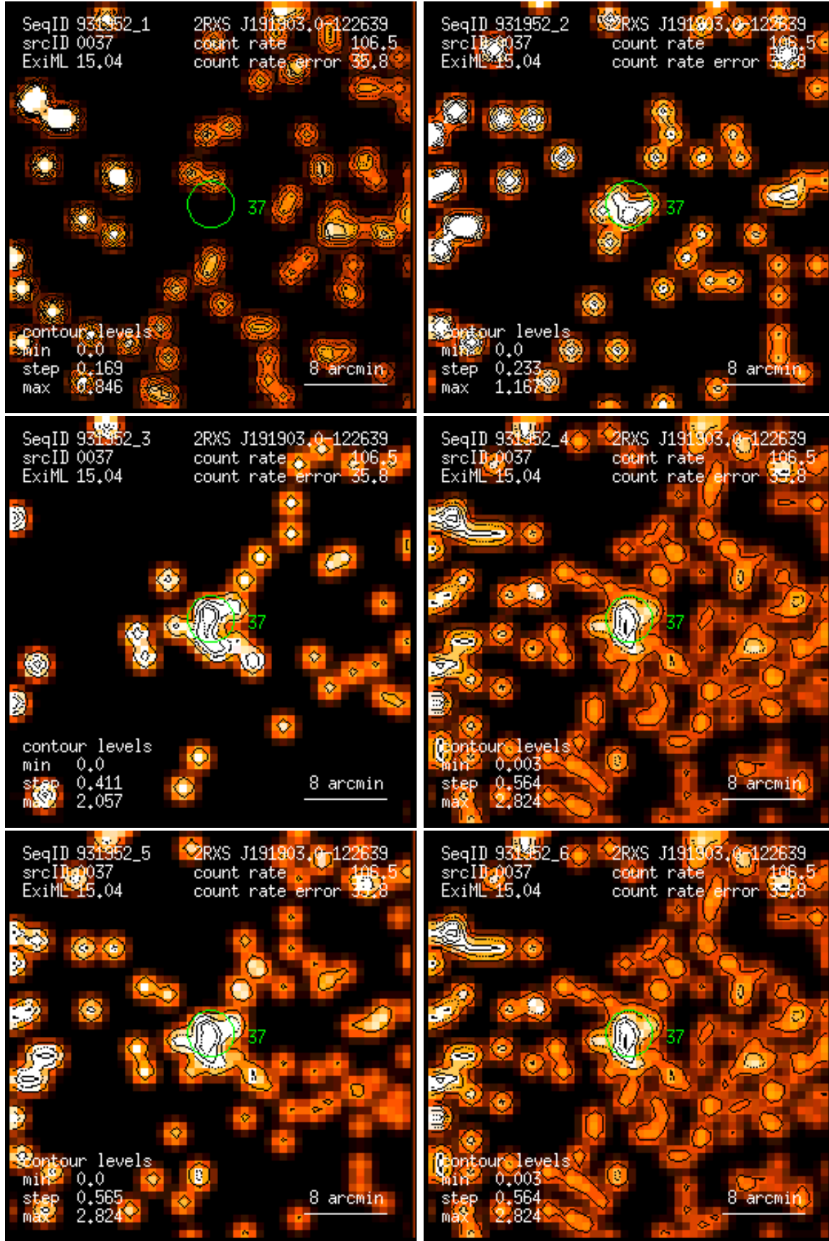
Figure 37: RASS 931952: detection 0037: band rate images, Gaussian filter: (1) PSPC channels 11 – 41, (2) 52 – 90, (3) 91 – 201, (4) 11 – 235, (5) 52 – 201, (6) 11 – 201. Broad band rates in counts/ks. Band rate contour levels in counts/ks/arcmin 2 .
