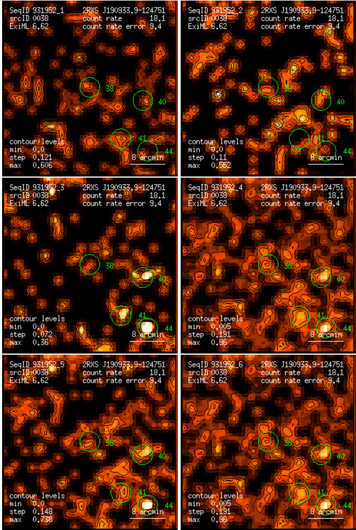
Figure 38: RASS 931952: detection 0038: band rate images, Gaussian filter: (1) PSPC channels 11 – 41, (2) 52 – 90, (3) 91 – 201, (4) 11 – 235, (5) 52 – 201, (6) 11 – 201. Broad band rates in counts/ks. Band rate contour levels in counts/ks/arcmin 2 .
