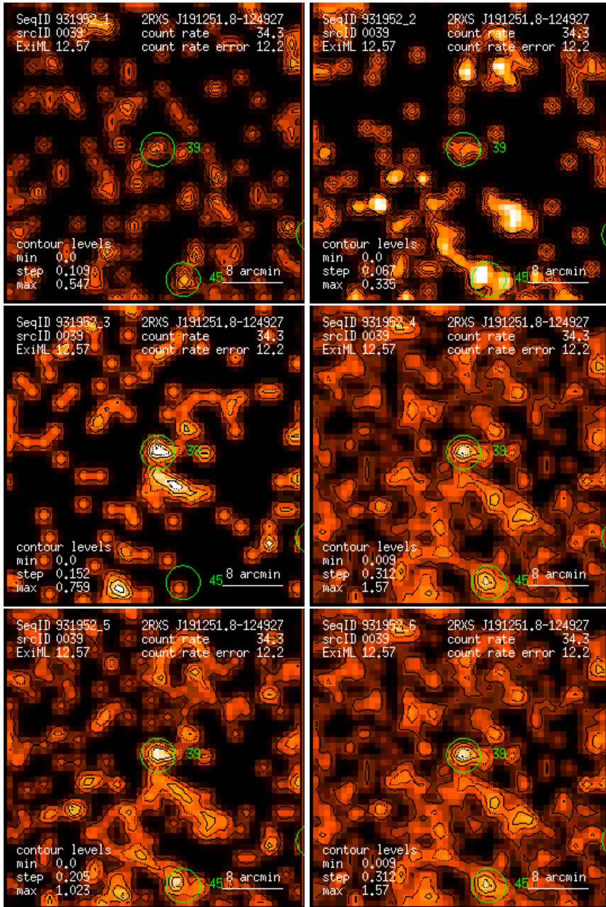
Figure 39: RASS 931952: detection 0039: band rate images, Gaussian filter: (1) PSPC channels 11 – 41, (2) 52 – 90, (3) 91 – 201, (4) 11 – 235, (5) 52 – 201, (6) 11 – 201. Broad band rates in counts/ks. Band rate contour levels in counts/ks/arcmin 2 .
