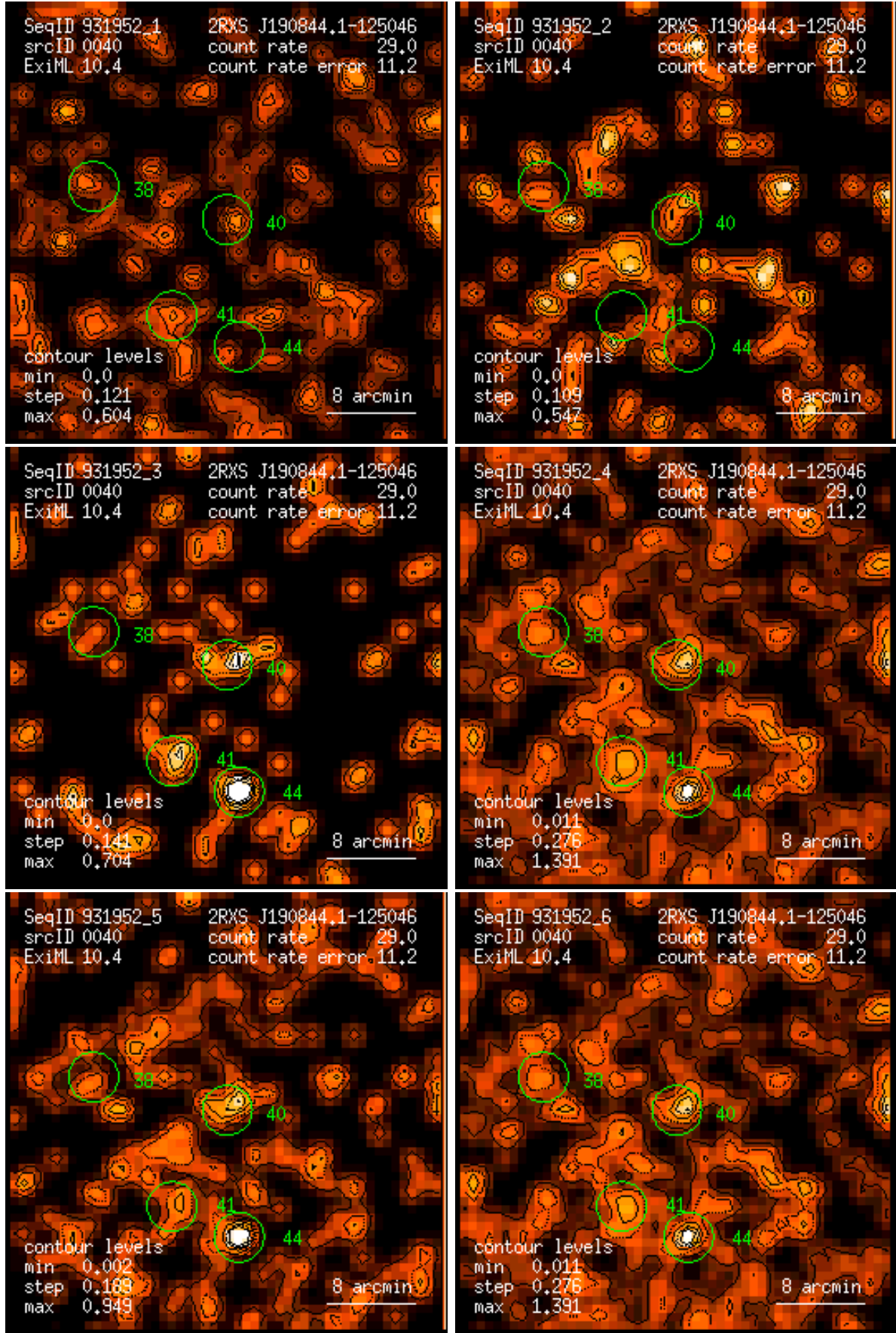
Figure 40: RASS 931952: detection 0040: band rate images, Gaussian filter: (1) PSPC channels 11 – 41, (2) 52 – 90, (3) 91 – 201, (4) 11 – 235, (5) 52 – 201, (6) 11 – 201. Broad band rates in counts/ks. Band rate contour levels in counts/ks/arcmin 2 .
