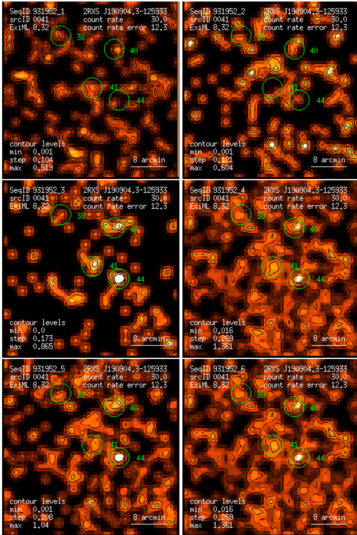
Figure 41: RASS 931952: detection 0041: band rate images, Gaussian filter: (1) PSPC channels 11 – 41, (2) 52 – 90, (3) 91 – 201, (4) 11 – 235, (5) 52 – 201, (6) 11 – 201. Broad band rates in counts/ks. Band rate contour levels in counts/ks/arcmin 2 .
