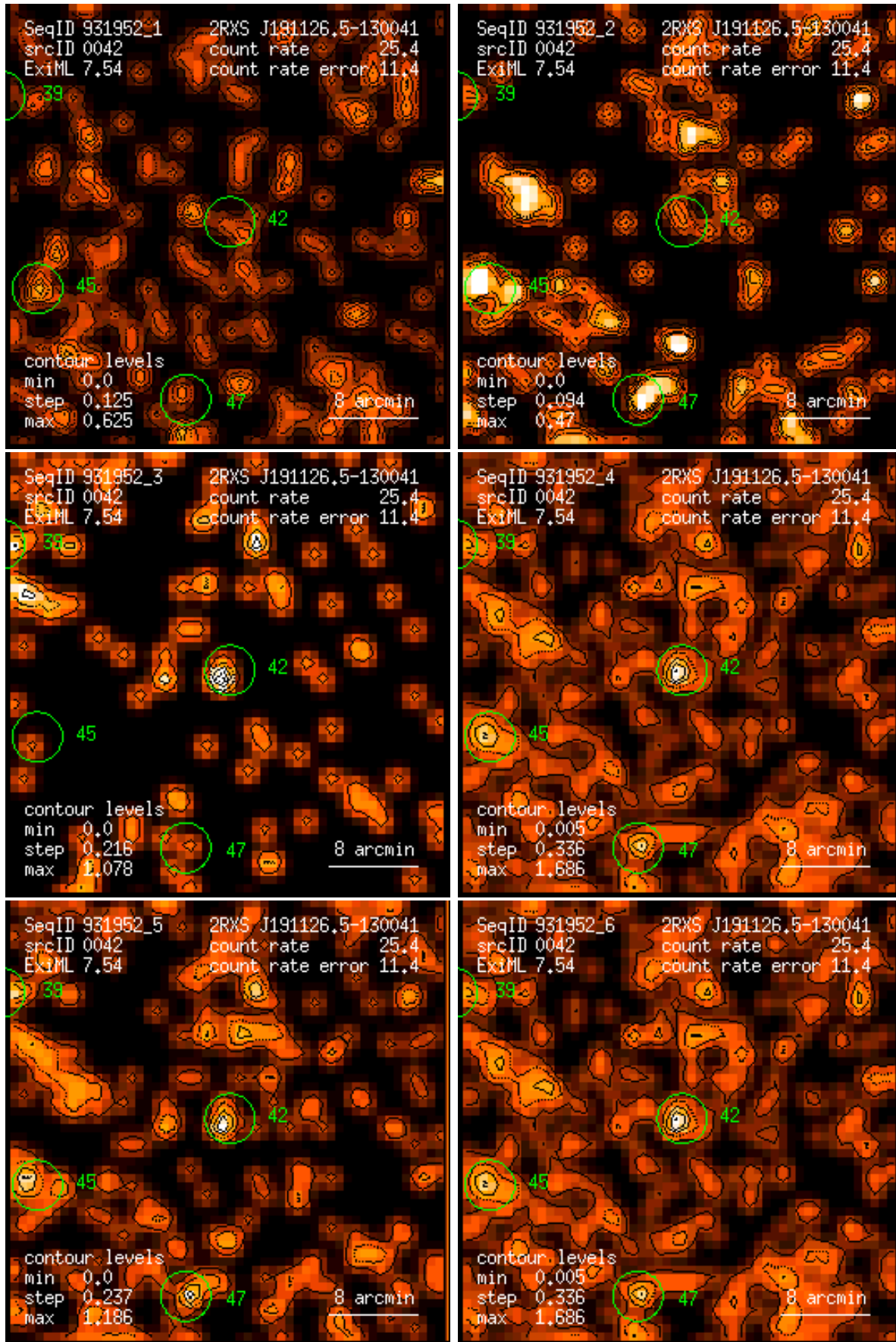
Figure 42: RASS 931952: detection 0042: band rate images, Gaussian filter: (1) PSPC channels 11 – 41, (2) 52 – 90, (3) 91 – 201, (4) 11 – 235, (5) 52 – 201, (6) 11 – 201. Broad band rates in counts/ks. Band rate contour levels in counts/ks/arcmin 2 .
