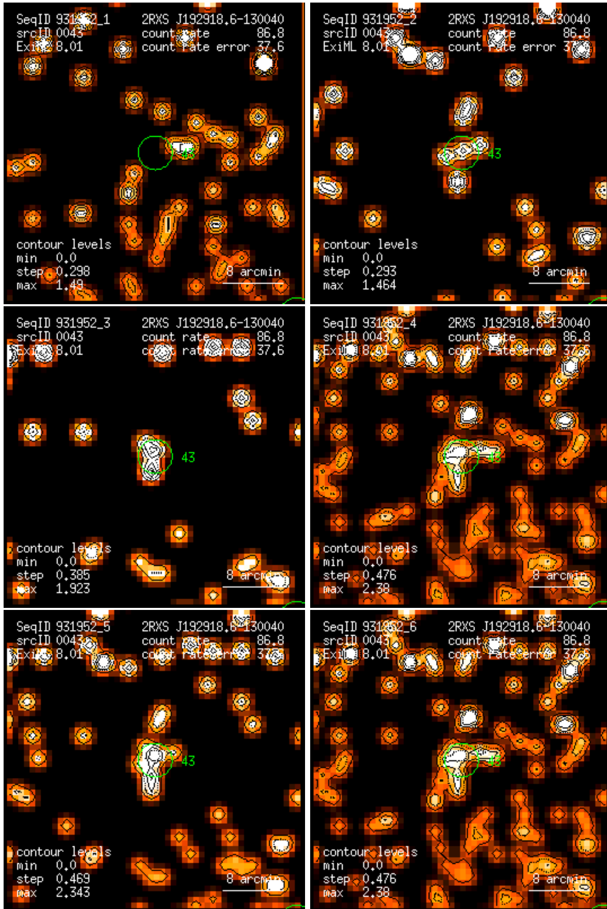
Figure 43: RASS 931952: detection 0043: band rate images, Gaussian filter: (1) PSPC channels 11 – 41, (2) 52 – 90, (3) 91 – 201, (4) 11 – 235, (5) 52 – 201, (6) 11 – 201. Broad band rates in counts/ks. Band rate contour levels in counts/ks/arcmin 2 .
