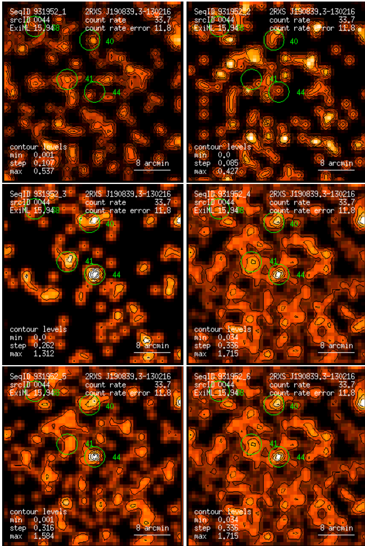
Figure 44: RASS 931952: detection 0044: band rate images, Gaussian filter: (1) PSPC channels 11 – 41, (2) 52 – 90, (3) 91 – 201, (4) 11 – 235, (5) 52 – 201, (6) 11 – 201. Broad band rates in counts/ks. Band rate contour levels in counts/ks/arcmin 2 .
