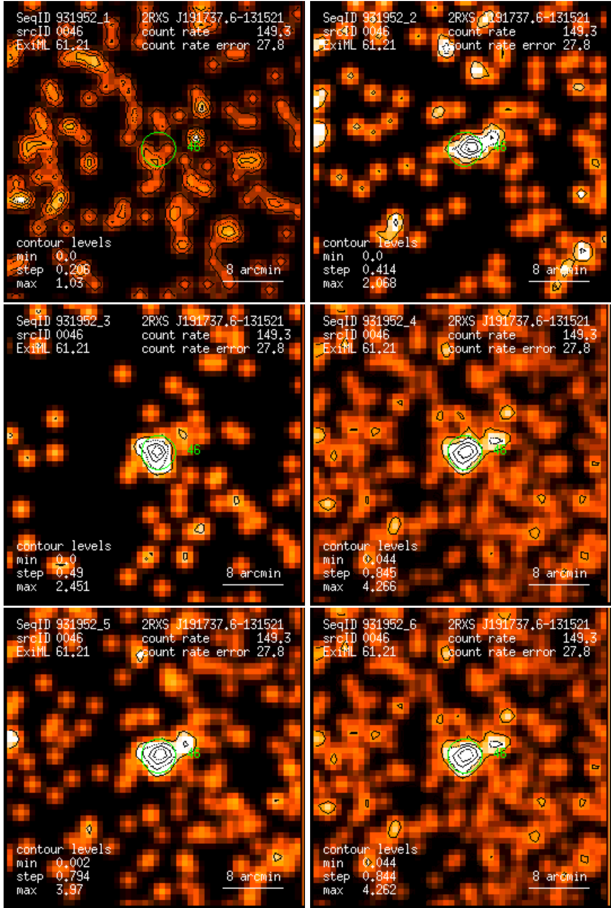
Figure 46: RASS 931952: detection 0046: band rate images, Gaussian filter: (1) PSPC channels 11 – 41, (2) 52 – 90, (3) 91 – 201, (4) 11 – 235, (5) 52 – 201, (6) 11 – 201. Broad band rates in counts/ks. Band rate contour levels in counts/ks/arcmin 2 .
