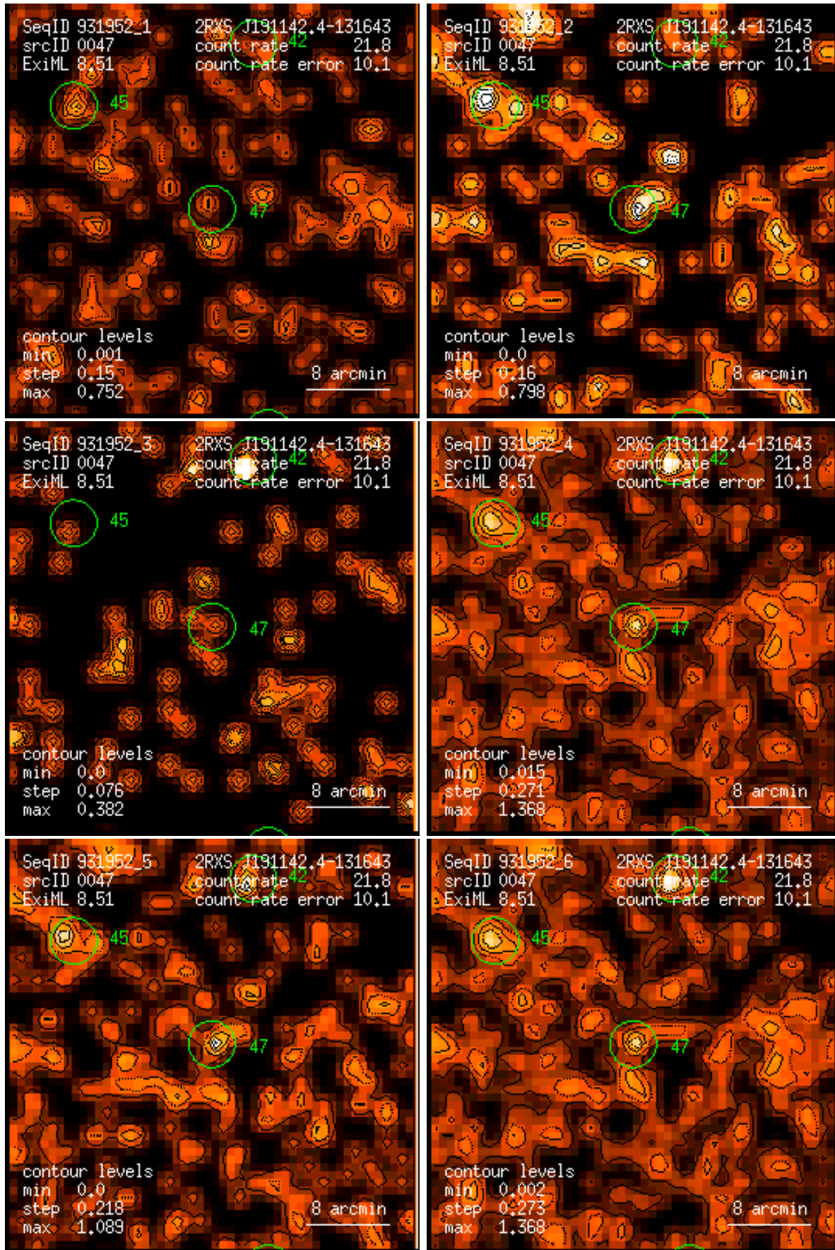
Figure 47: RASS 931952: detection 0047: band rate images, Gaussian filter: (1) PSPC channels 11 – 41, (2) 52 – 90, (3) 91 – 201, (4) 11 – 235, (5) 52 – 201, (6) 11 – 201. Broad band rates in counts/ks. Band rate contour levels in counts/ks/arcmin 2 .
