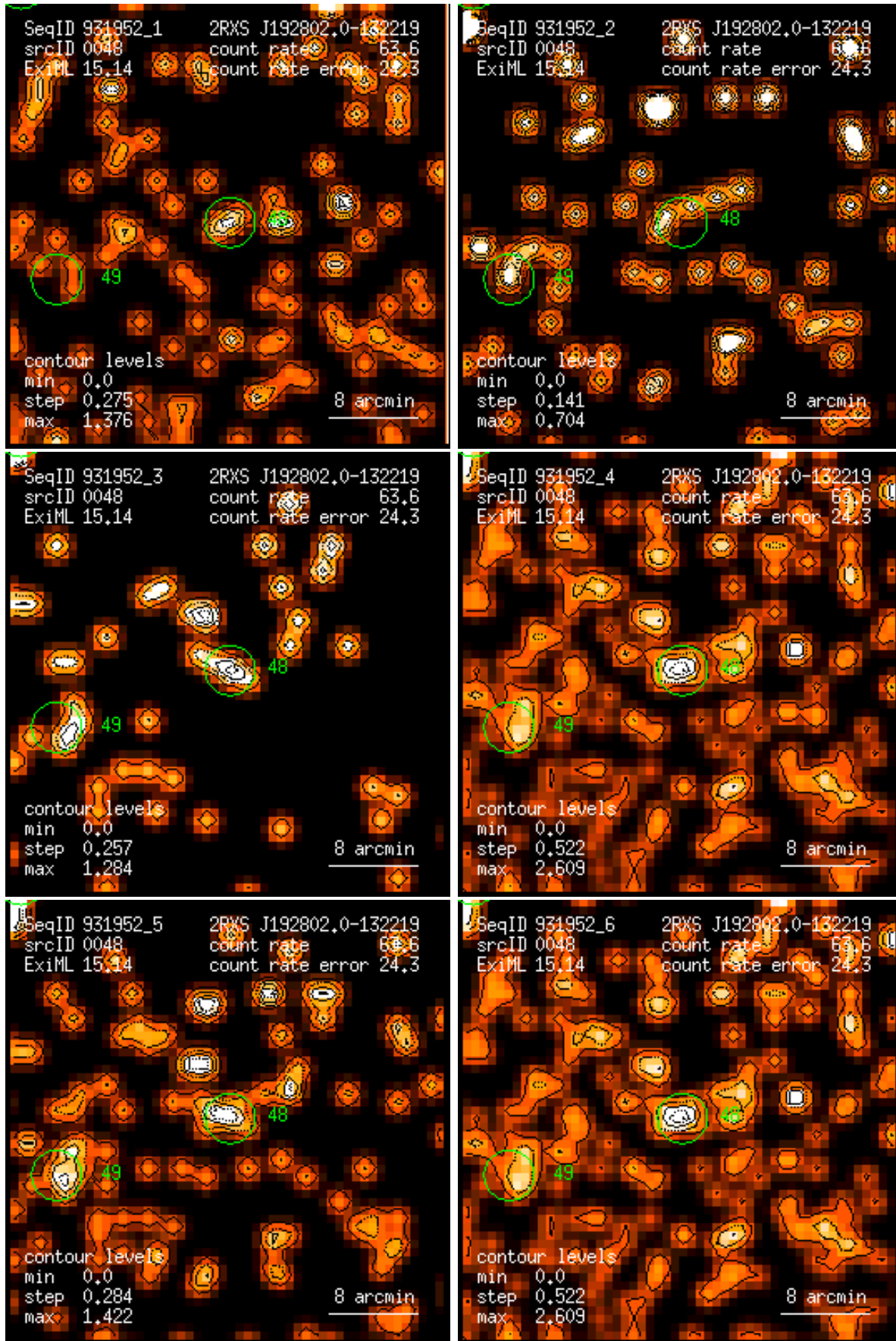
Figure 48: RASS 931952: detection 0048: band rate images, Gaussian filter: (1) PSPC channels 11 – 41, (2) 52 – 90, (3) 91 – 201, (4) 11 – 235, (5) 52 – 201, (6) 11 – 201. Broad band rates in counts/ks. Band rate contour levels in counts/ks/arcmin 2 .
