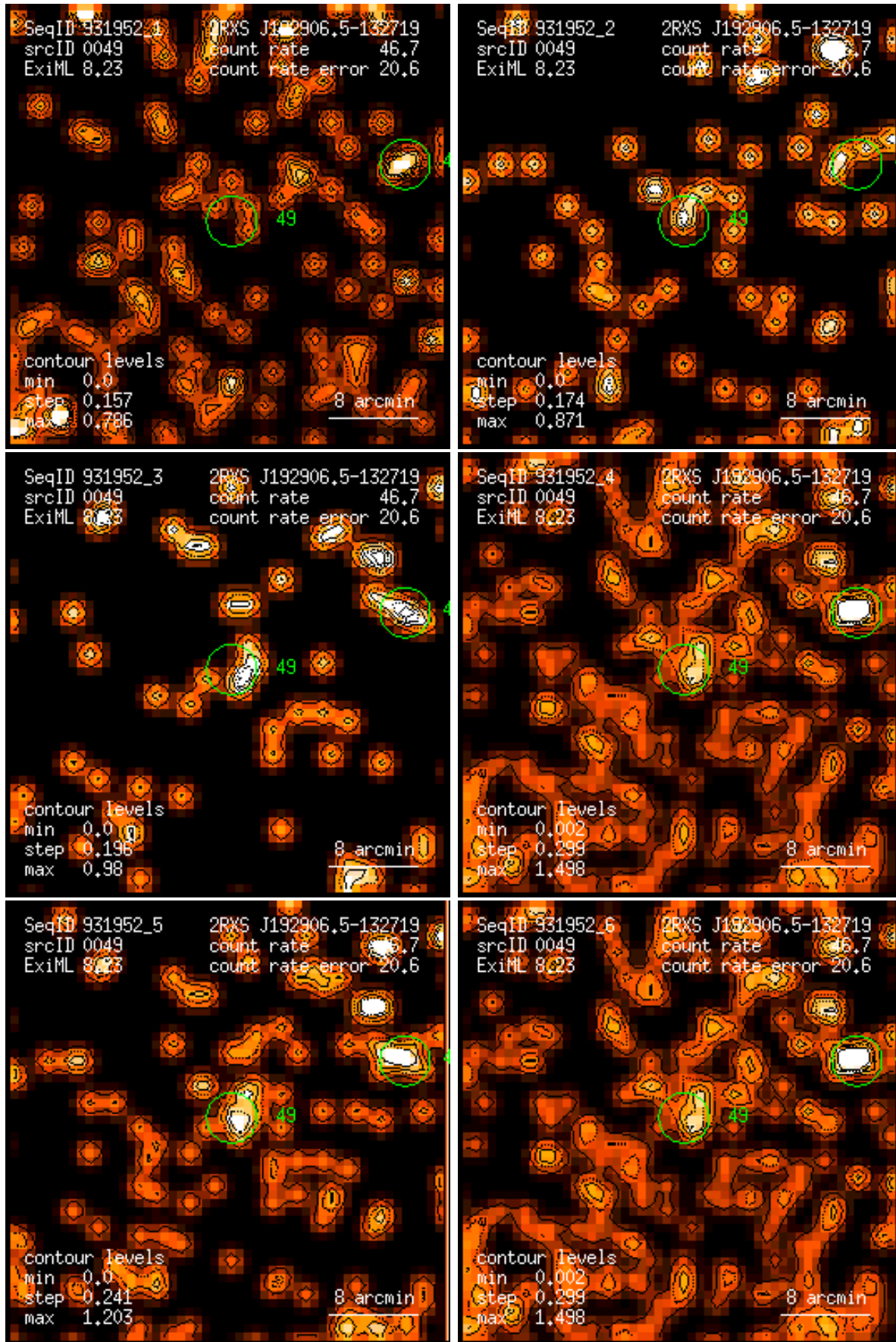
Figure 49: RASS 931952: detection 0049: band rate images, Gaussian filter: (1) PSPC channels 11 – 41, (2) 52 – 90, (3) 91 – 201, (4) 11 – 235, (5) 52 – 201, (6) 11 – 201. Broad band rates in counts/ks. Band rate contour levels in counts/ks/arcmin 2 .
