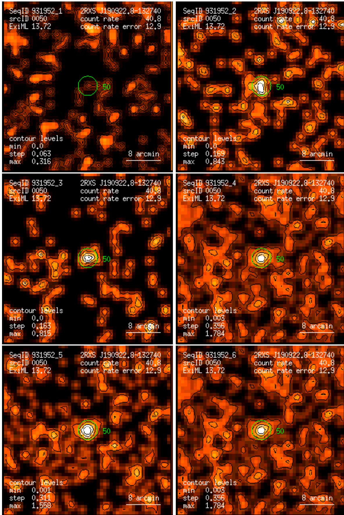
Figure 50: RASS 931952: detection 0050: band rate images, Gaussian filter: (1) PSPC channels 11 – 41, (2) 52 – 90, (3) 91 – 201, (4) 11 – 235, (5) 52 – 201, (6) 11 – 201. Broad band rates in counts/ks. Band rate contour levels in counts/ks/arcmin 2 .
