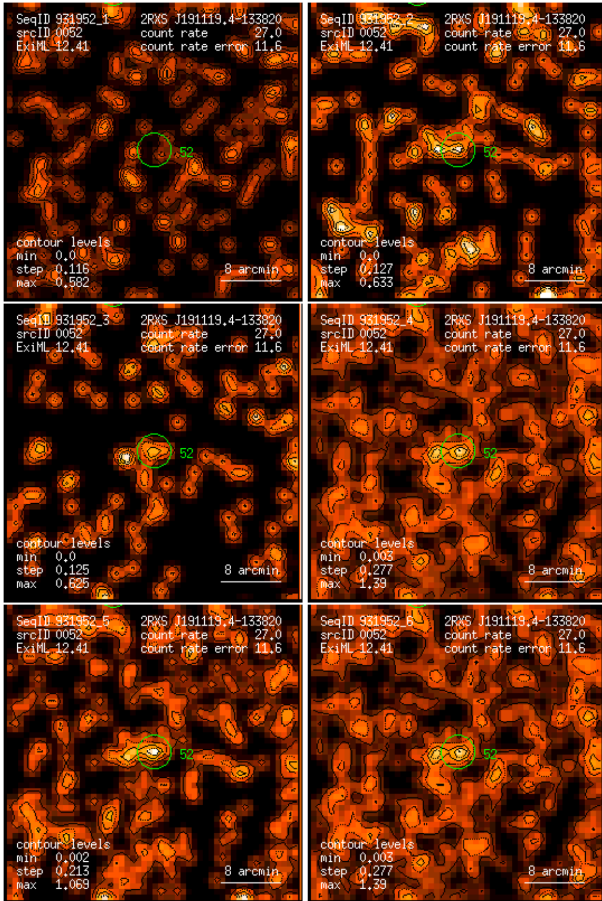
Figure 52: RASS 931952: detection 0052: band rate images, Gaussian filter: (1) PSPC channels 11 – 41, (2) 52 – 90, (3) 91 – 201, (4) 11 – 235, (5) 52 – 201, (6) 11 – 201. Broad band rates in counts/ks. Band rate contour levels in counts/ks/arcmin 2 .
