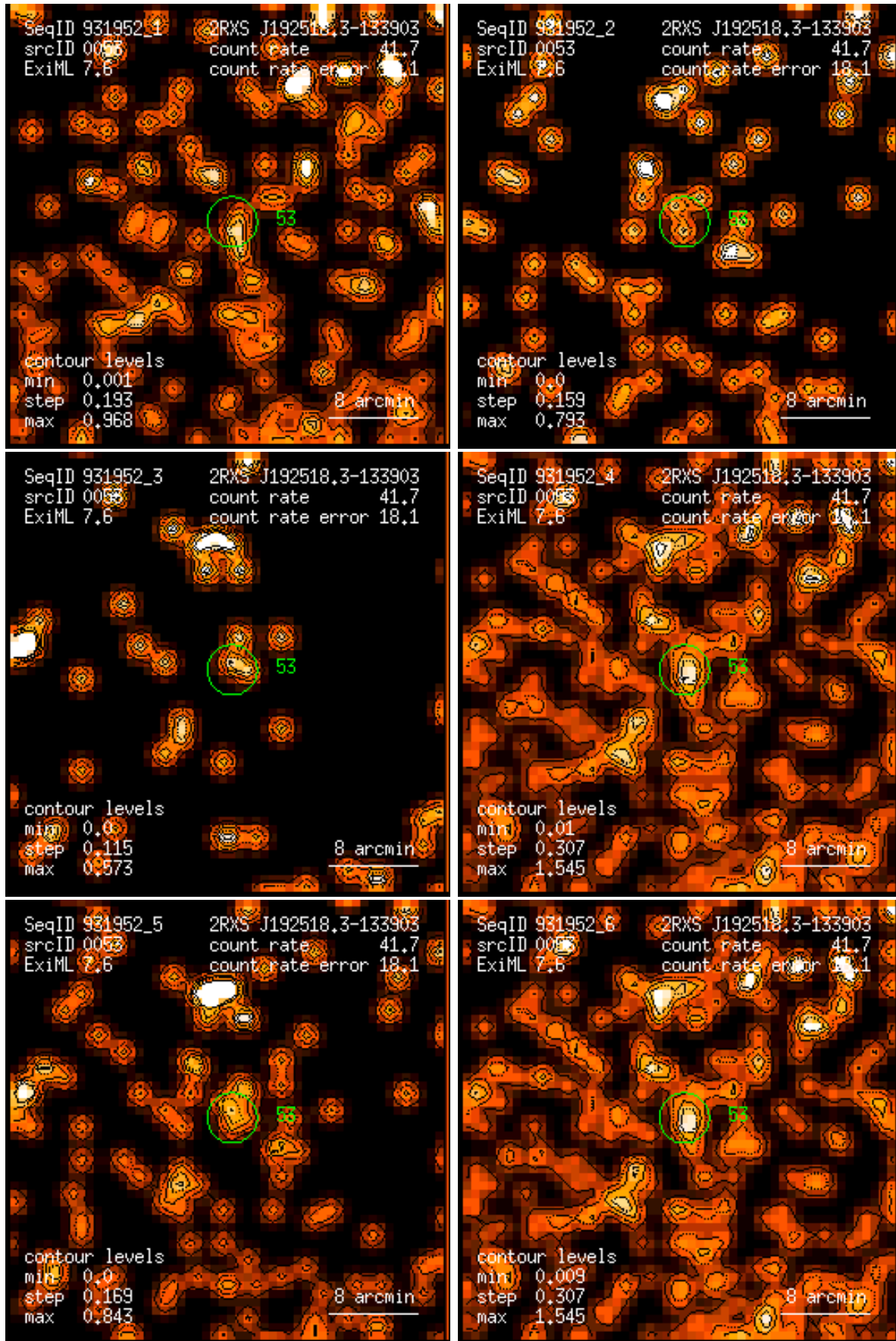
Figure 53: RASS 931952: detection 0053: band rate images, Gaussian filter: (1) PSPC channels 11 – 41, (2) 52 – 90, (3) 91 – 201, (4) 11 – 235, (5) 52 – 201, (6) 11 – 201. Broad band rates in counts/ks. Band rate contour levels in counts/ks/arcmin 2 .
