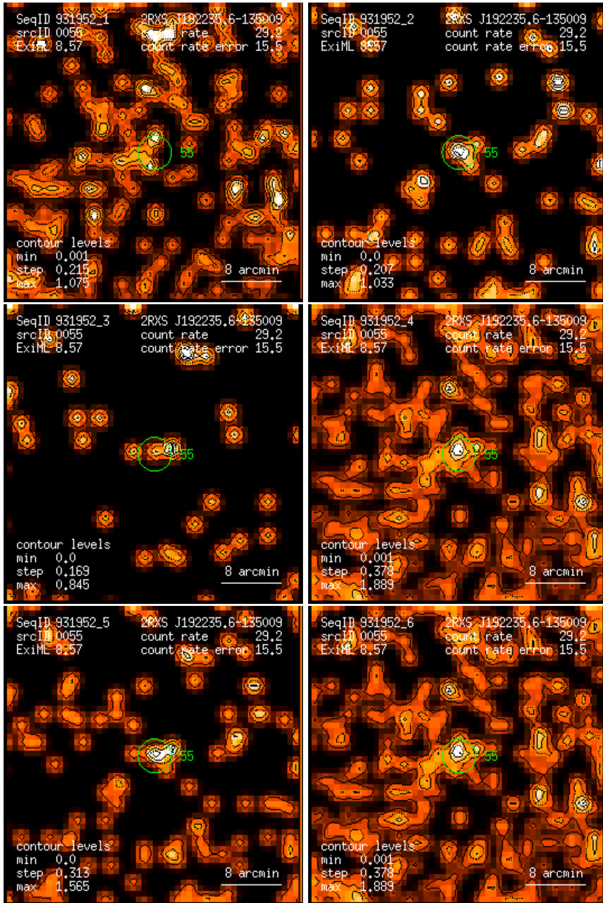
Figure 55: RASS 931952: detection 0055: band rate images, Gaussian filter: (1) PSPC channels 11 – 41, (2) 52 – 90, (3) 91 – 201, (4) 11 – 235, (5) 52 – 201, (6) 11 – 201. Broad band rates in counts/ks. Band rate contour levels in counts/ks/arcmin 2 .
