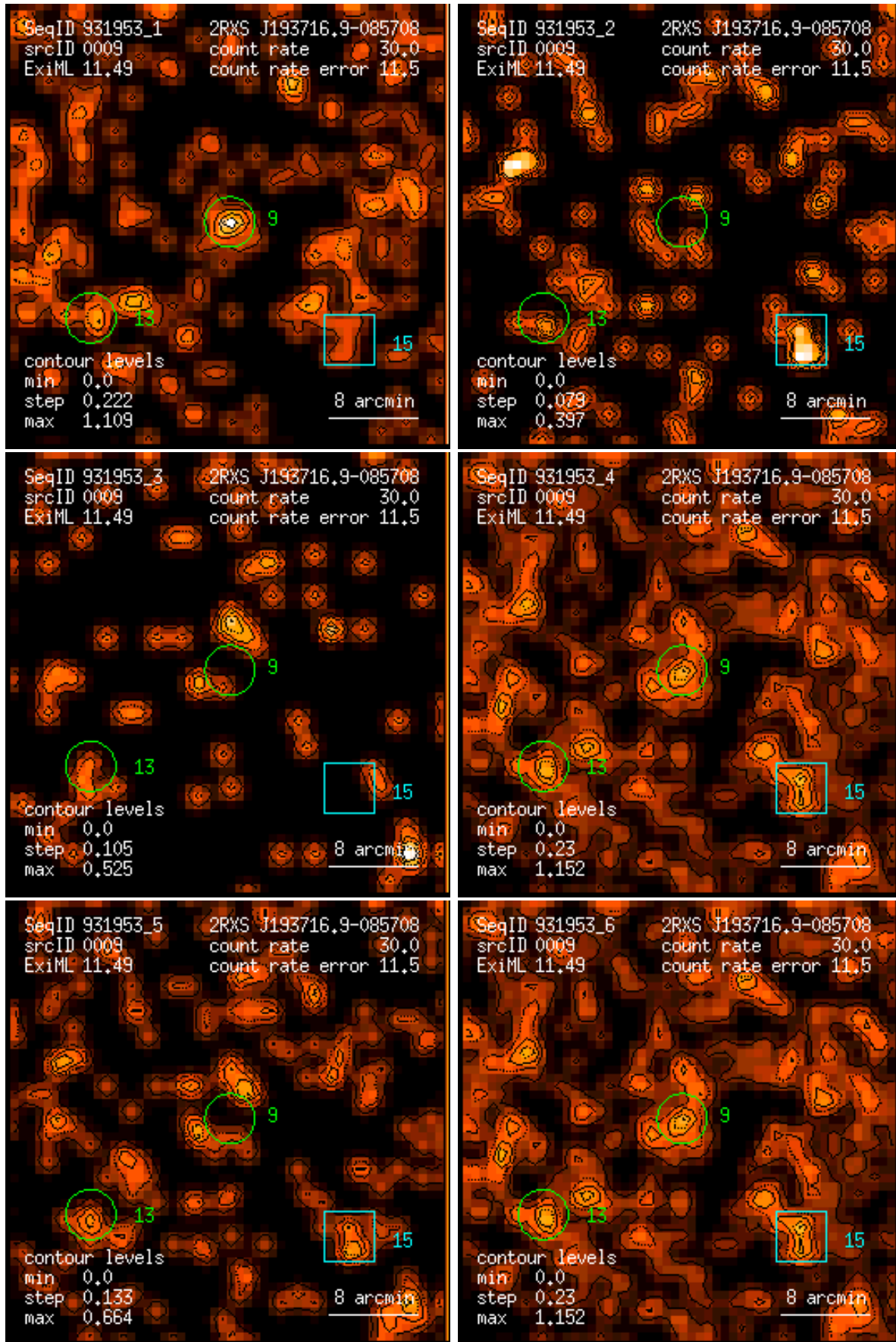
Figure 9: RASS 931953: detection 0009: band rate images, Gaussian filter: (1) PSPC channels 11 – 41, (2) 52 – 90, (3) 91 – 201, (4) 11 – 235, (5) 52 – 201, (6) 11 – 201. Broad band rates in counts/ks. Band rate contour levels in counts/ks/arcmin 2 .
