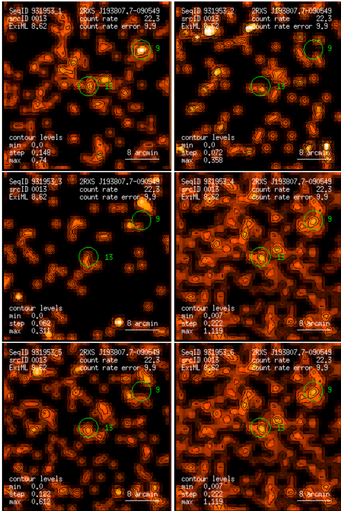
Figure 13: RASS 931953: detection 0013: band rate images, Gaussian filter: (1) PSPC channels 11 – 41, (2) 52 – 90, (3) 91 – 201, (4) 11 – 235, (5) 52 – 201, (6) 11 – 201. Broad band rates in counts/ks. Band rate contour levels in counts/ks/arcmin 2 .
