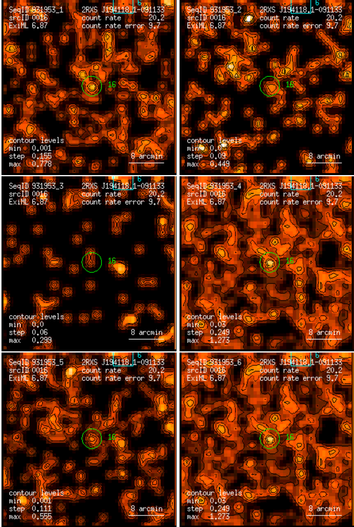
Figure 16: RASS 931953: detection 0016: band rate images, Gaussian filter: (1) PSPC channels 11 – 41, (2) 52 – 90, (3) 91 – 201, (4) 11 – 235, (5) 52 – 201, (6) 11 – 201. Broad band rates in counts/ks. Band rate contour levels in counts/ks/arcmin 2 .
