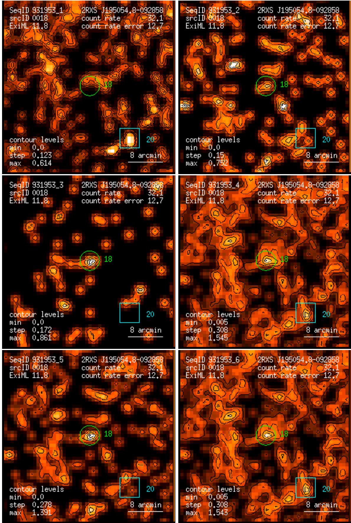
Figure 18: RASS 931953: detection 0018: band rate images, Gaussian filter: (1) PSPC channels 11 – 41, (2) 52 – 90, (3) 91 – 201, (4) 11 – 235, (5) 52 – 201, (6) 11 – 201. Broad band rates in counts/ks. Band rate contour levels in counts/ks/arcmin 2 .
