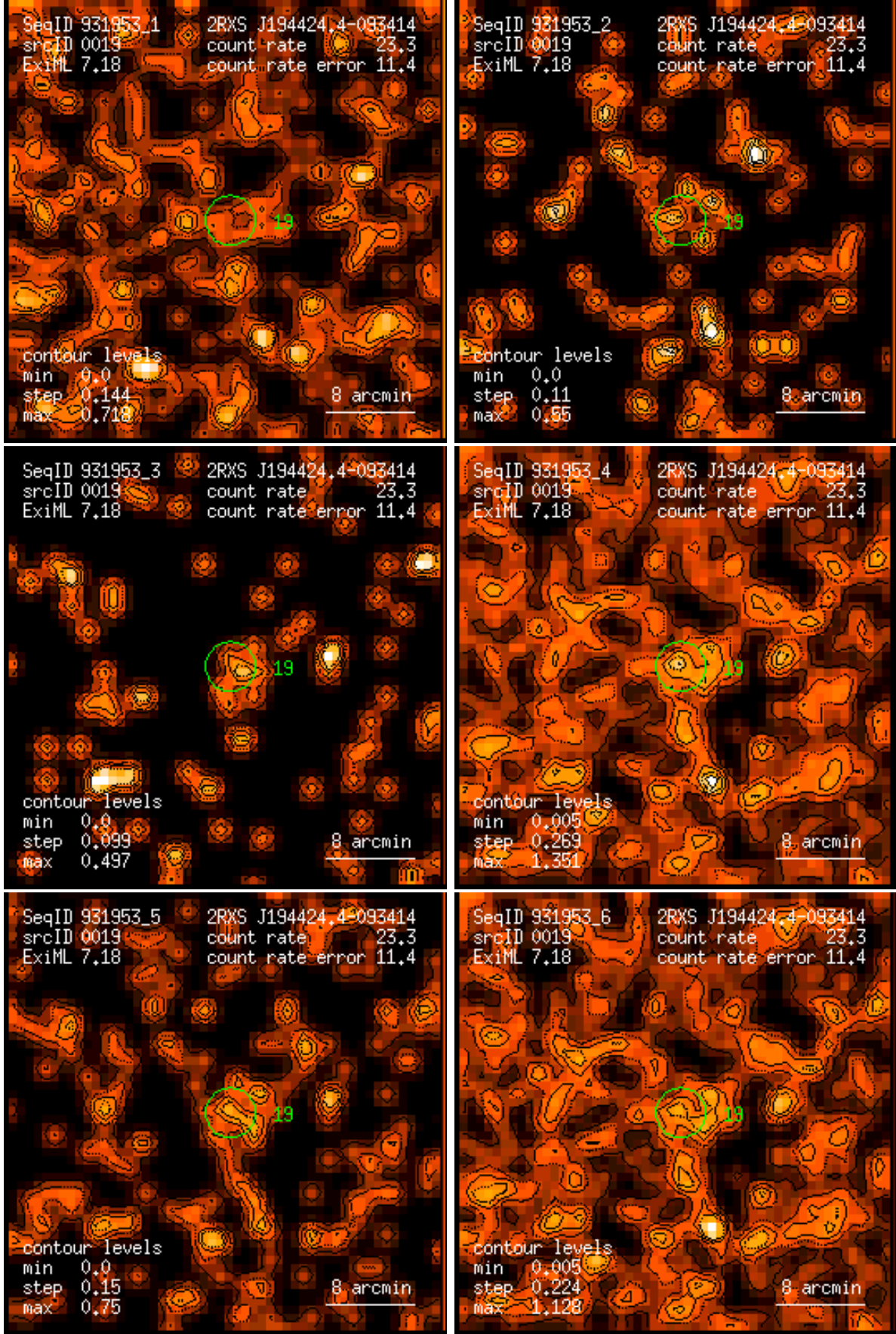
Figure 19: RASS 931953: detection 0019: band rate images, Gaussian filter: (1) PSPC channels 11 – 41, (2) 52 – 90, (3) 91 – 201, (4) 11 – 235, (5) 52 – 201, (6) 11 – 201. Broad band rates in counts/ks. Band rate contour levels in counts/ks/arcmin 2 .
