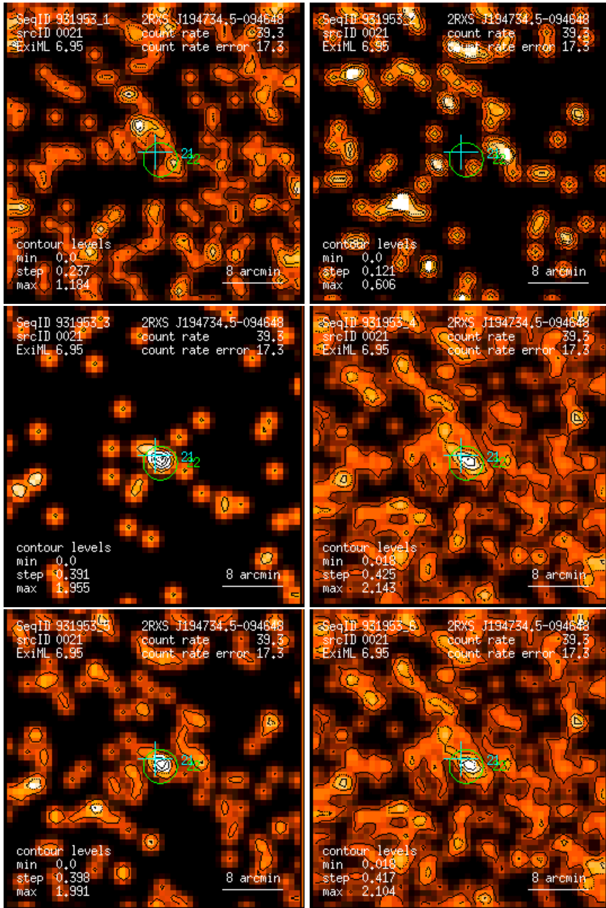
Figure 21: RASS 931953: detection 0021: band rate images, Gaussian filter: (1) PSPC channels 11 – 41, (2) 52 – 90, (3) 91 – 201, (4) 11 – 235, (5) 52 – 201, (6) 11 – 201. Broad band rates in counts/ks. Band rate contour levels in counts/ks/arcmin 2 .
