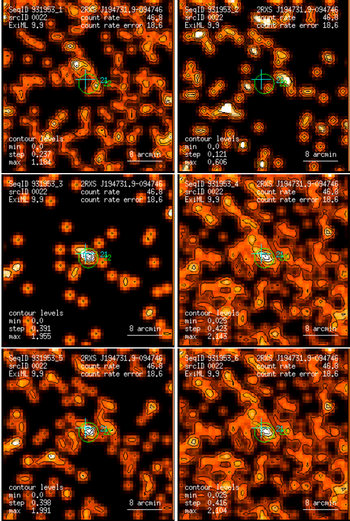
Figure 22: RASS 931953: detection 0022: band rate images, Gaussian filter: (1) PSPC channels 11 – 41, (2) 52 – 90, (3) 91 – 201, (4) 11 – 235, (5) 52 – 201, (6) 11 – 201. Broad band rates in counts/ks. Band rate contour levels in counts/ks/arcmin 2 .
