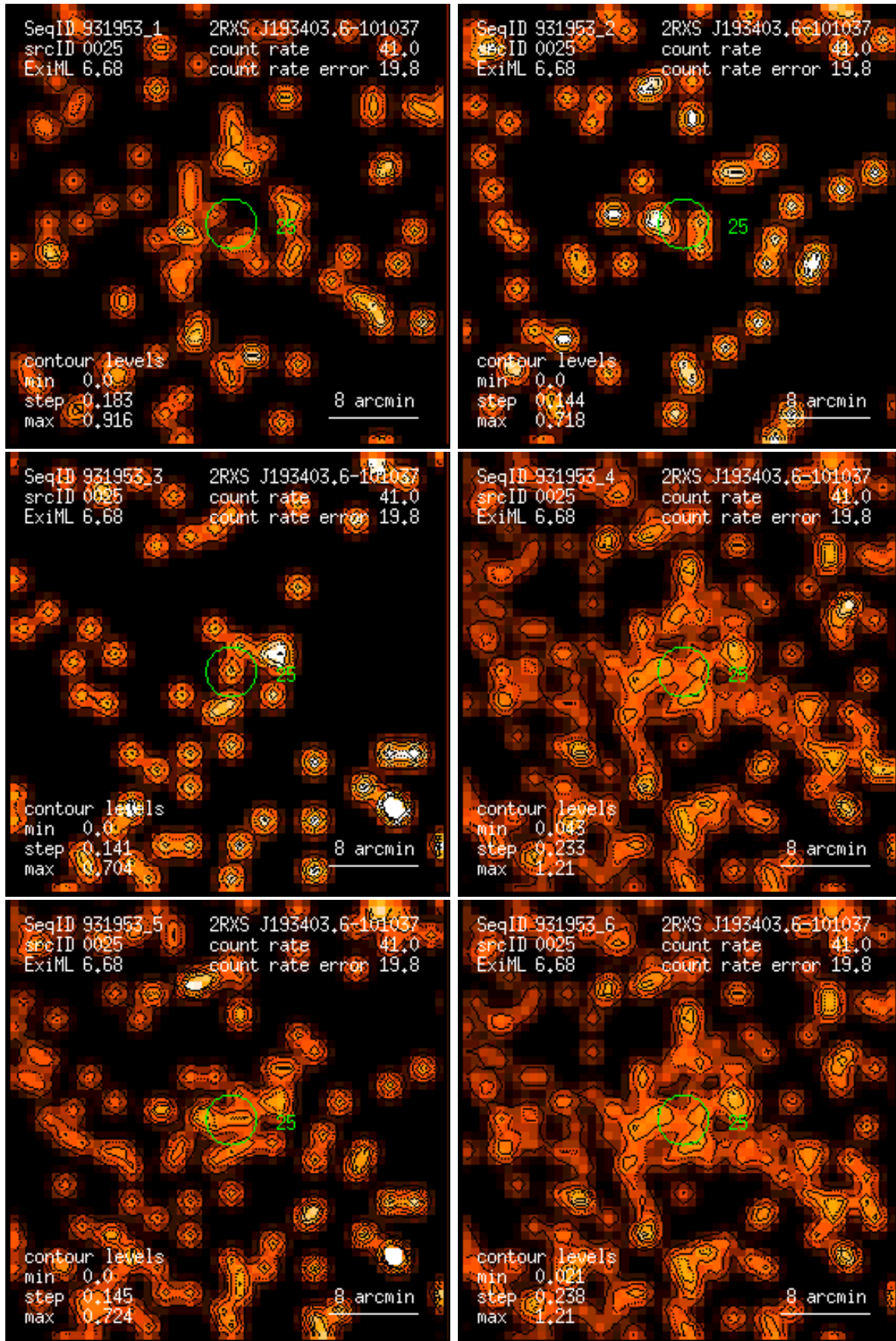
Figure 25: RASS 931953: detection 0025: band rate images, Gaussian filter: (1) PSPC channels 11 – 41, (2) 52 – 90, (3) 91 – 201, (4) 11 – 235, (5) 52 – 201, (6) 11 – 201. Broad band rates in counts/ks. Band rate contour levels in counts/ks/arcmin 2 .
