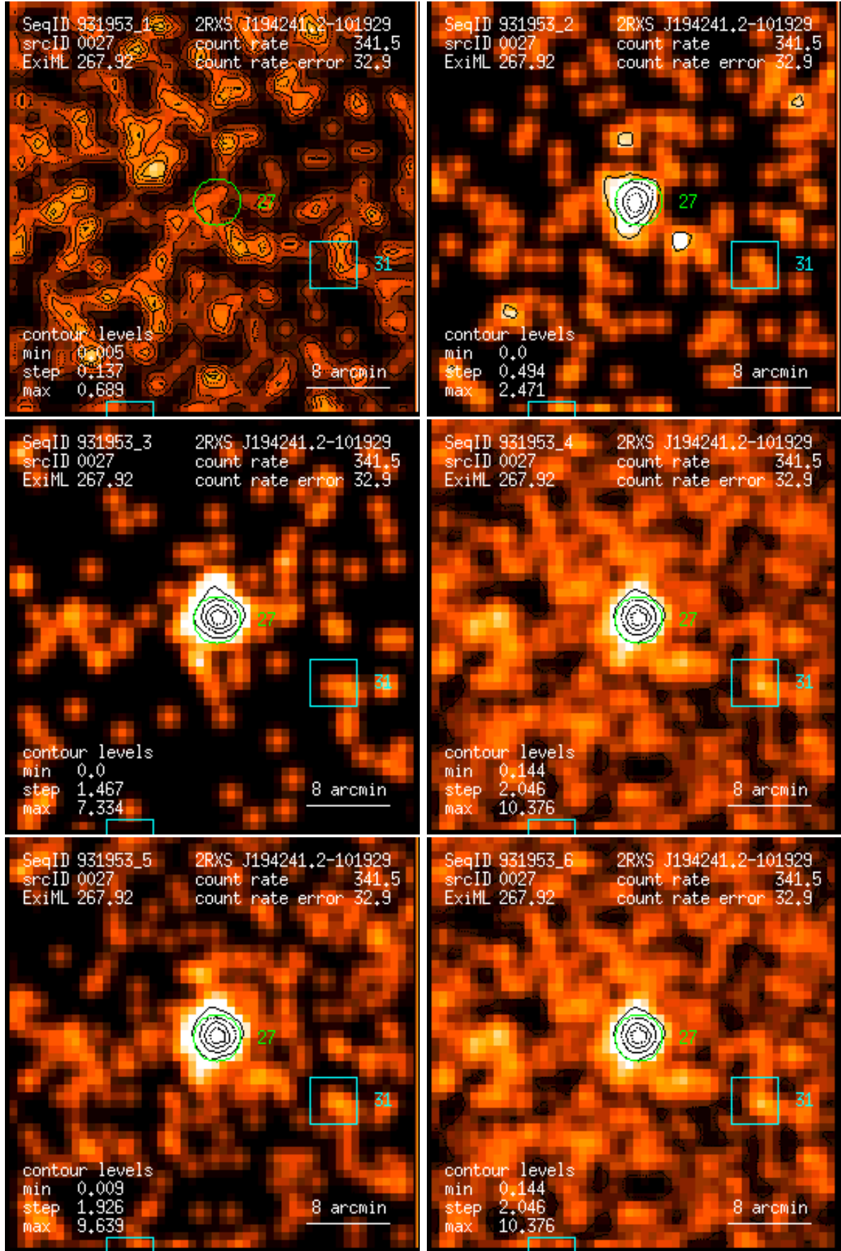
Figure 27: RASS 931953: detection 0027: band rate images, Gaussian filter: (1) PSPC channels 11 – 41, (2) 52 – 90, (3) 91 – 201, (4) 11 – 235, (5) 52 – 201, (6) 11 – 201. Broad band rates in counts/ks. Band rate contour levels in counts/ks/arcmin 2 .
