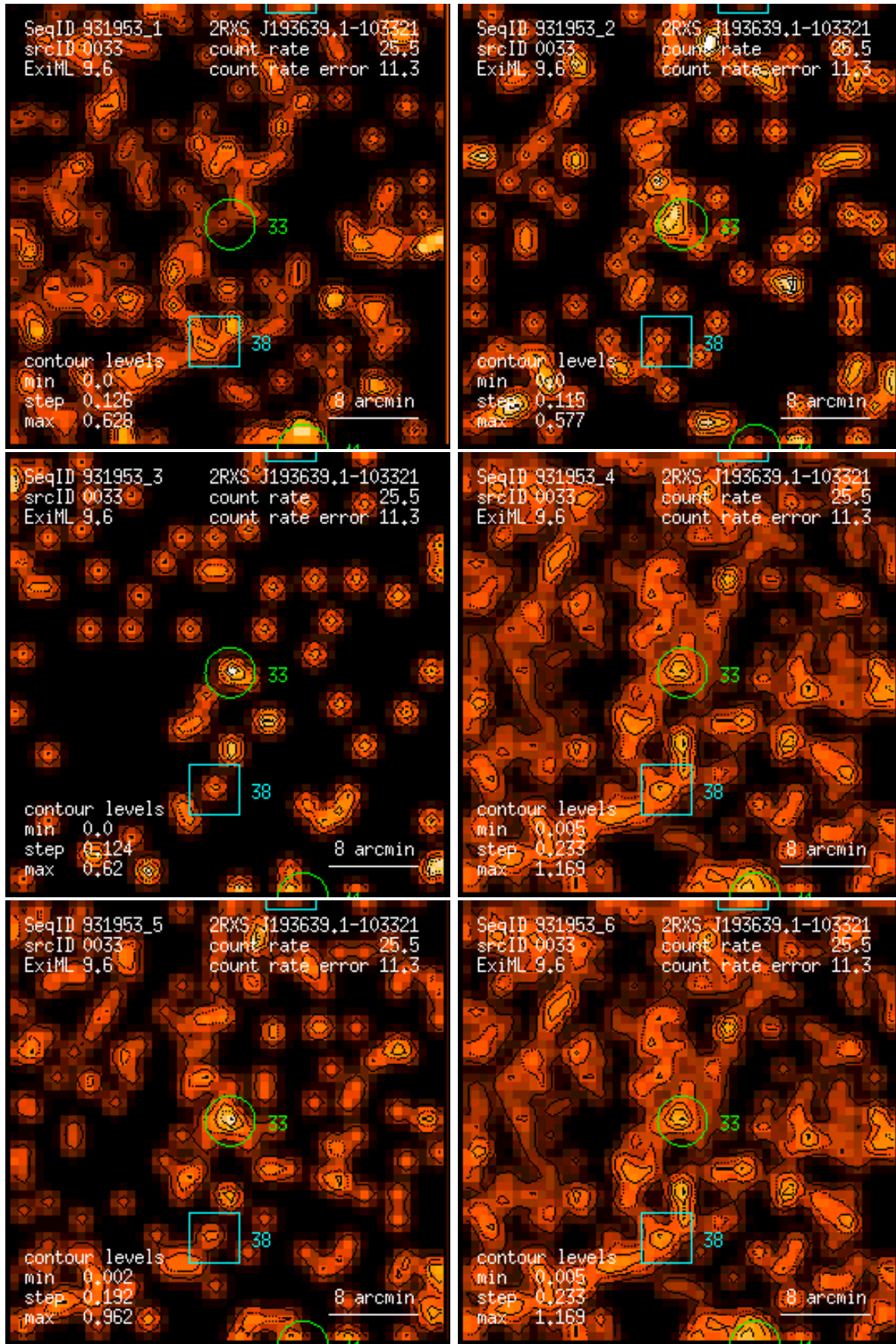
Figure 33: RASS 931953: detection 0033: band rate images, Gaussian filter: (1) PSPC channels 11 – 41, (2) 52 – 90, (3) 91 – 201, (4) 11 – 235, (5) 52 – 201, (6) 11 – 201. Broad band rates in counts/ks. Band rate contour levels in counts/ks/arcmin 2 .
