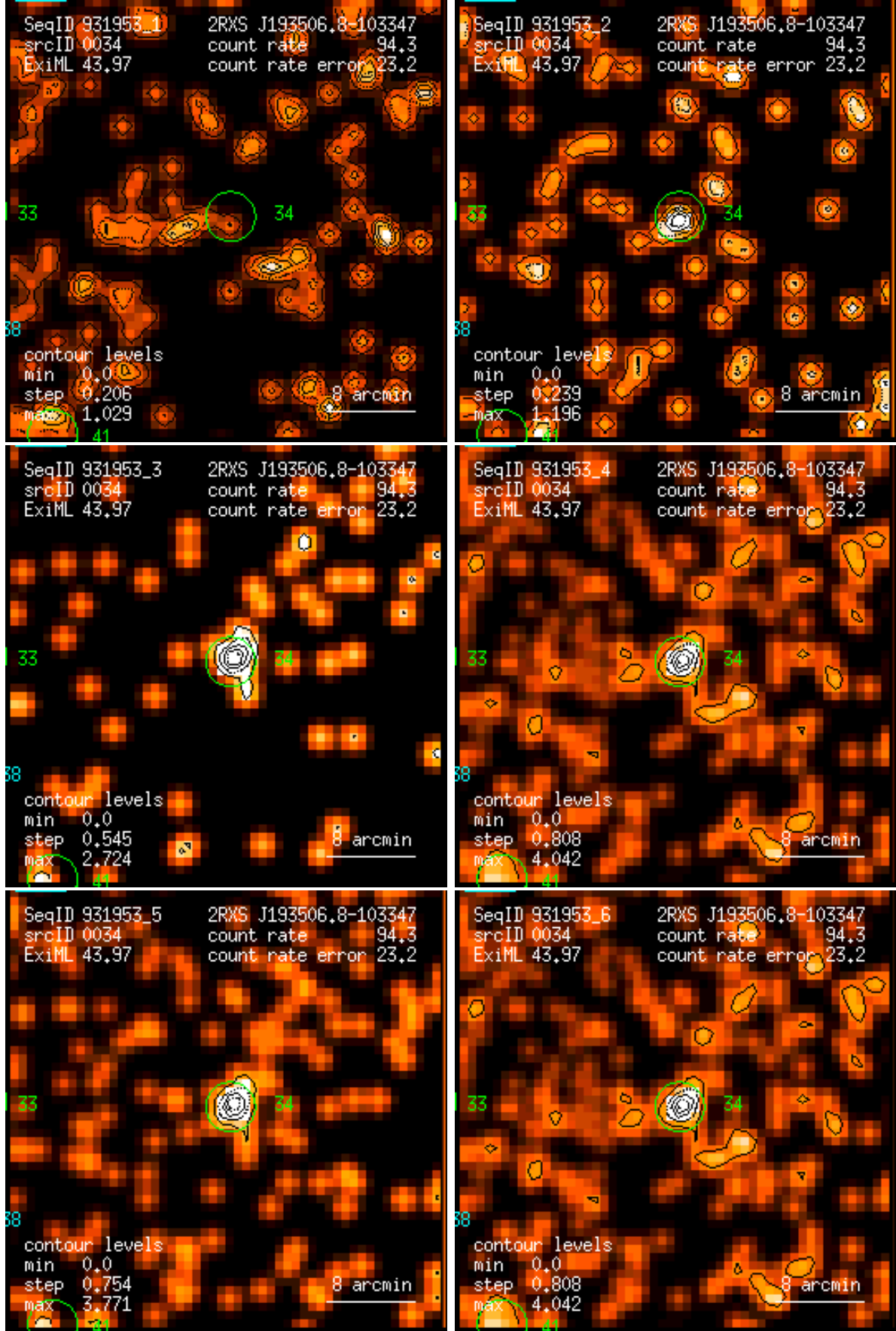
Figure 34: RASS 931953: detection 0034: band rate images, Gaussian filter: (1) PSPC channels 11 – 41, (2) 52 – 90, (3) 91 – 201, (4) 11 – 235, (5) 52 – 201, (6) 11 – 201. Broad band rates in counts/ks. Band rate contour levels in counts/ks/arcmin 2 .
