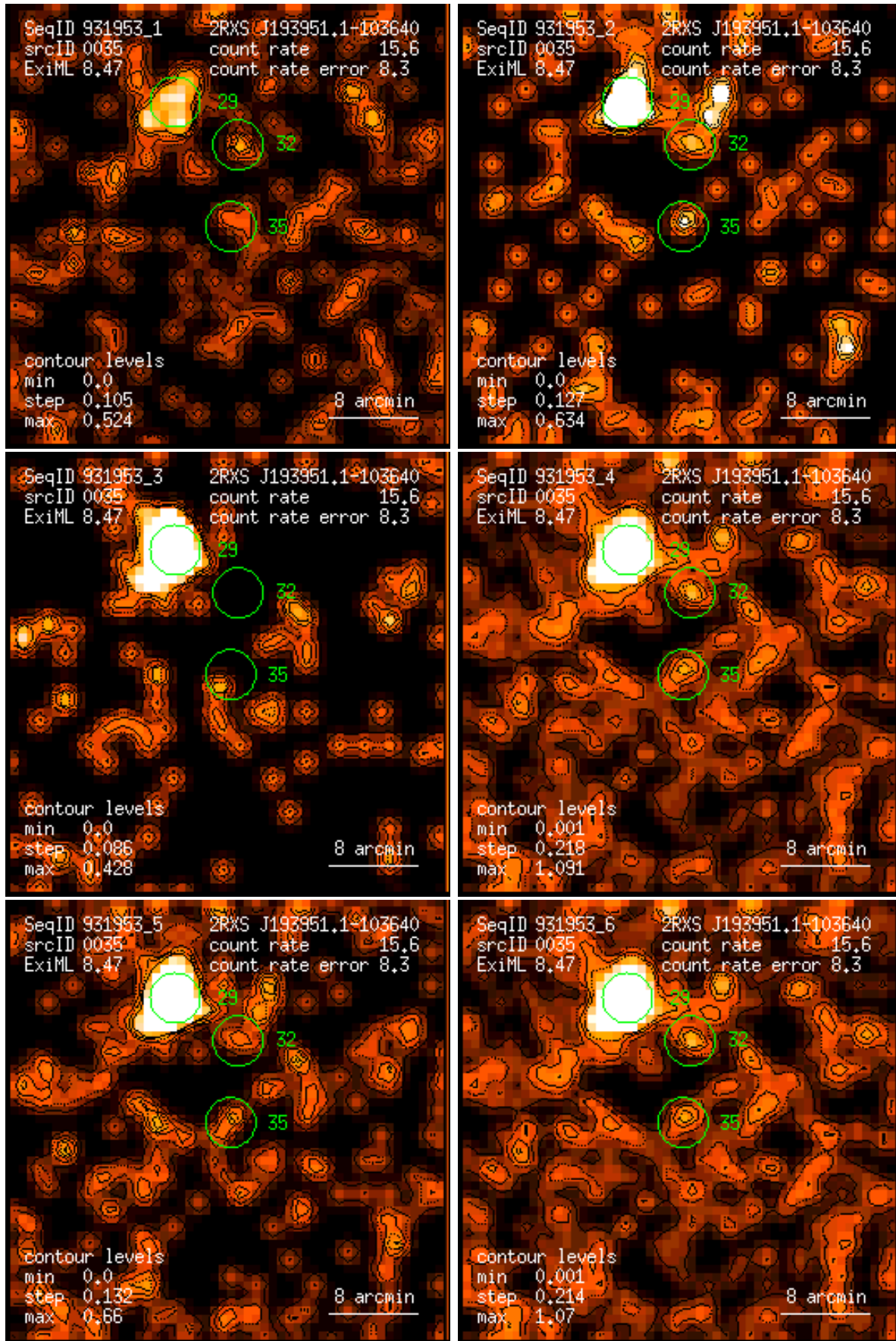
Figure 35: RASS 931953: detection 0035: band rate images, Gaussian filter: (1) PSPC channels 11 – 41, (2) 52 – 90, (3) 91 – 201, (4) 11 – 235, (5) 52 – 201, (6) 11 – 201. Broad band rates in counts/ks. Band rate contour levels in counts/ks/arcmin 2 .
