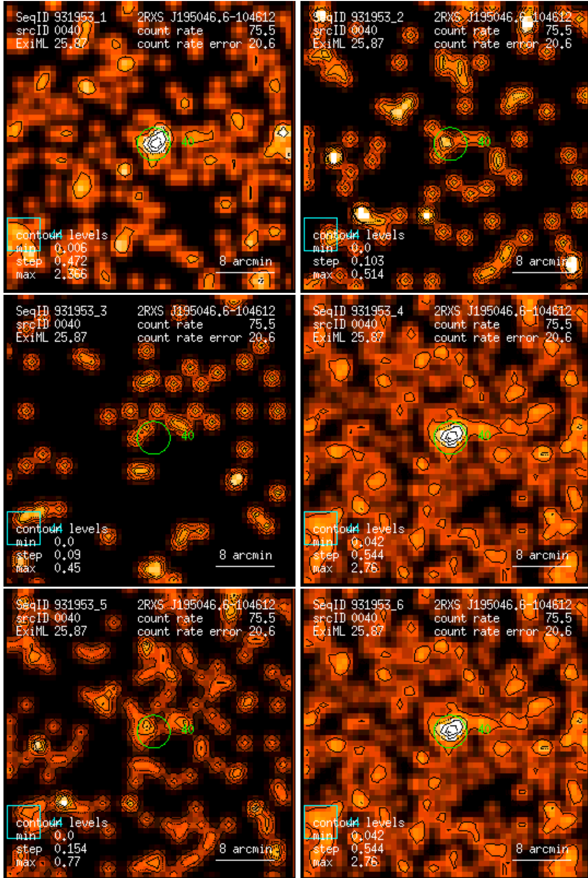
Figure 40: RASS 931953: detection 0040: band rate images, Gaussian filter: (1) PSPC channels 11 – 41, (2) 52 – 90, (3) 91 – 201, (4) 11 – 235, (5) 52 – 201, (6) 11 – 201. Broad band rates in counts/ks. Band rate contour levels in counts/ks/arcmin 2 .
