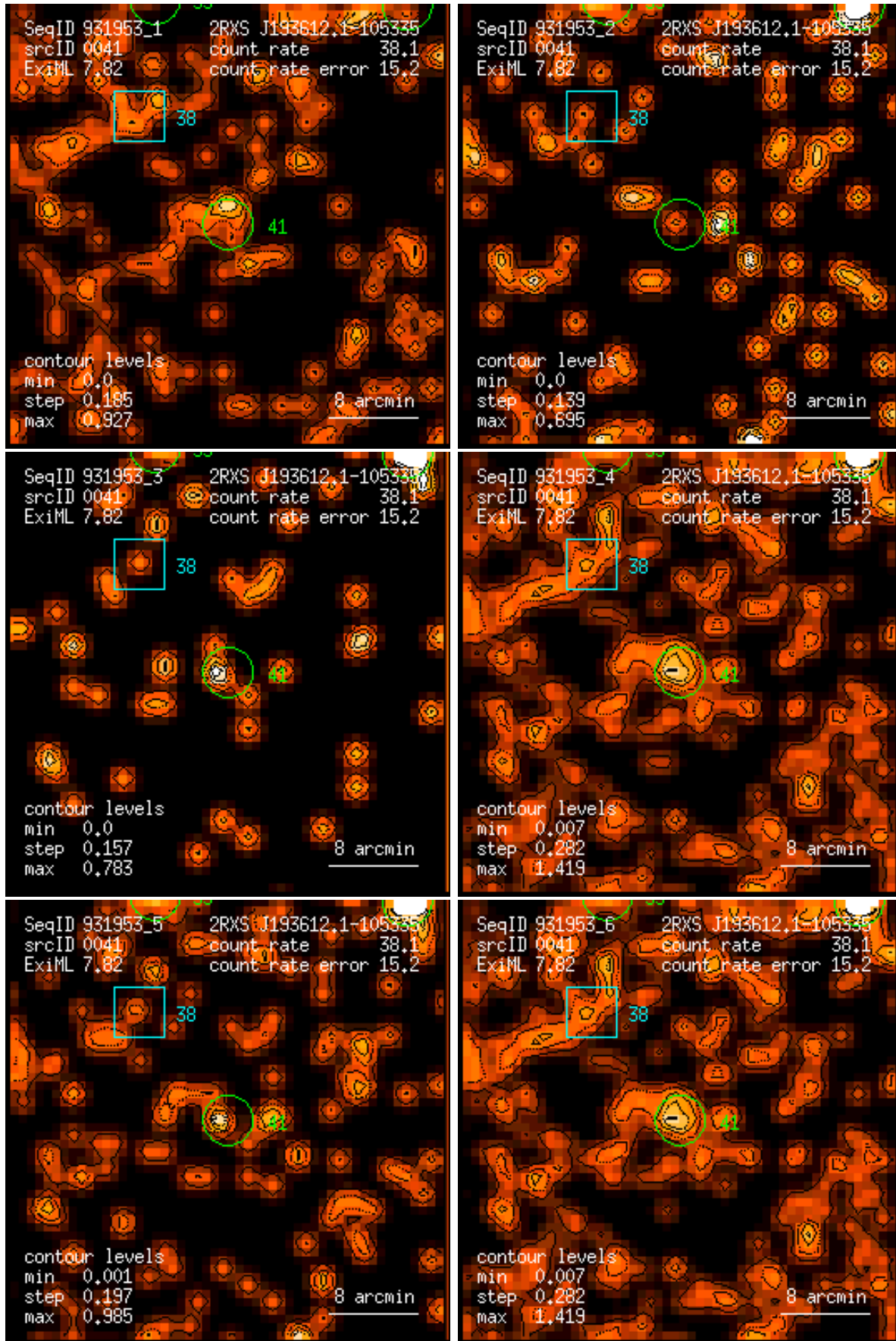
Figure 41: RASS 931953: detection 0041: band rate images, Gaussian filter: (1) PSPC channels 11 – 41, (2) 52 – 90, (3) 91 – 201, (4) 11 – 235, (5) 52 – 201, (6) 11 – 201. Broad band rates in counts/ks. Band rate contour levels in counts/ks/arcmin 2 .
