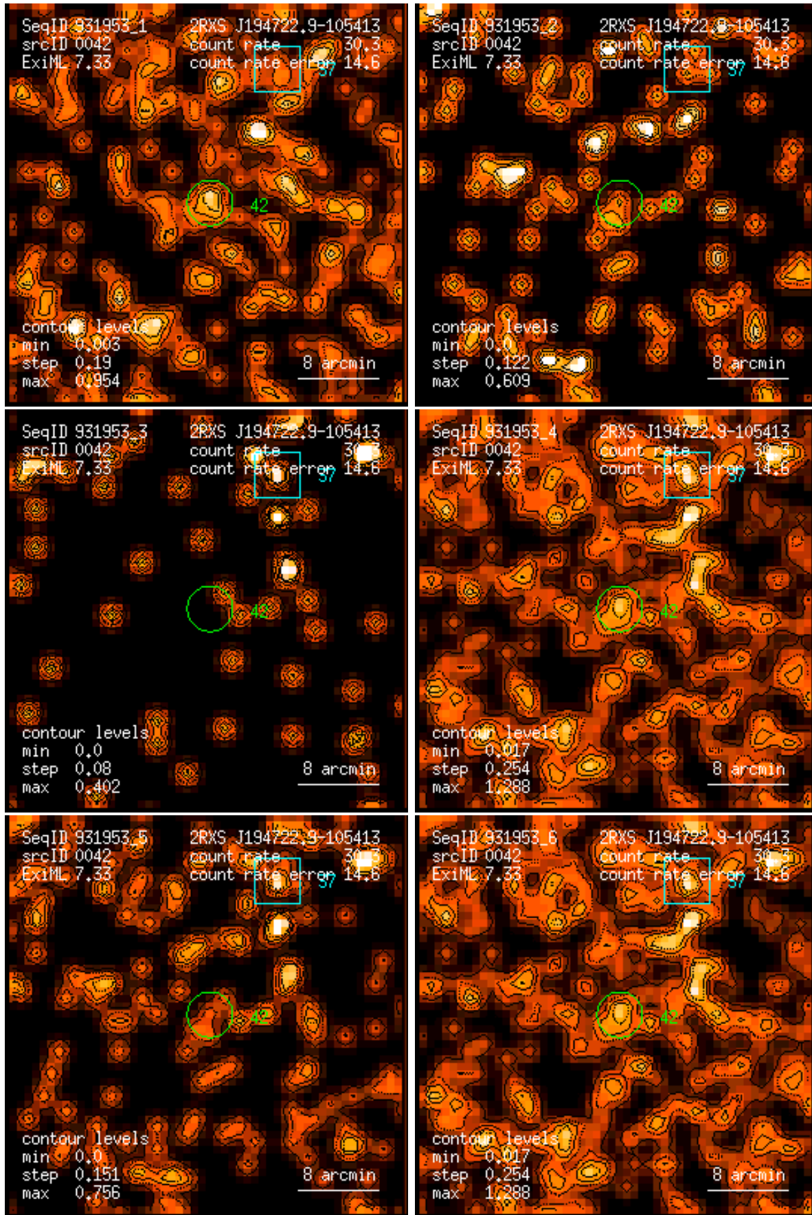
Figure 42: RASS 931953: detection 0042: band rate images, Gaussian filter: (1) PSPC channels 11 – 41, (2) 52 – 90, (3) 91 – 201, (4) 11 – 235, (5) 52 – 201, (6) 11 – 201. Broad band rates in counts/ks. Band rate contour levels in counts/ks/arcmin 2 .
